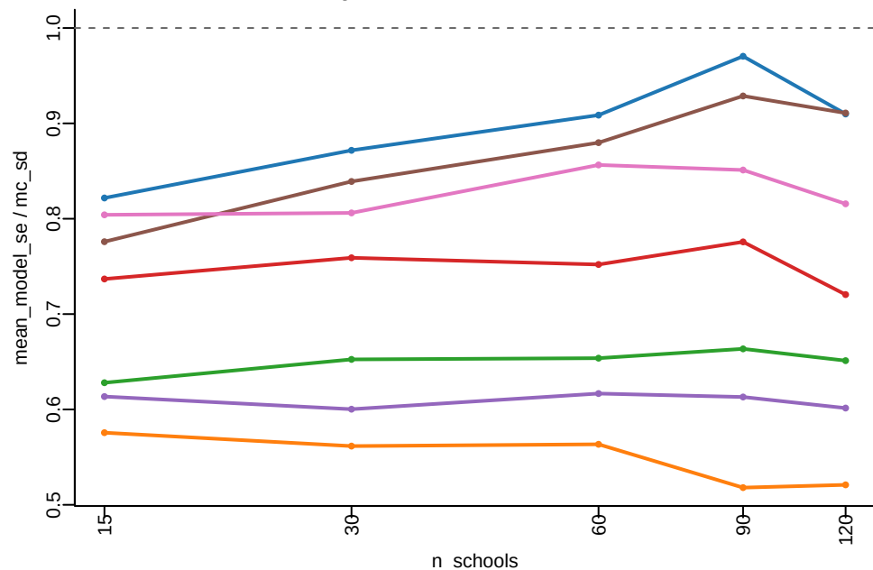
Model A_synth : Fixed-Effect SE Calibration
