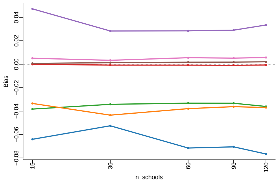
Model A_synth : Variance-Component Bias
