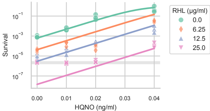
Linear Logit Model in RHL and HQNO
