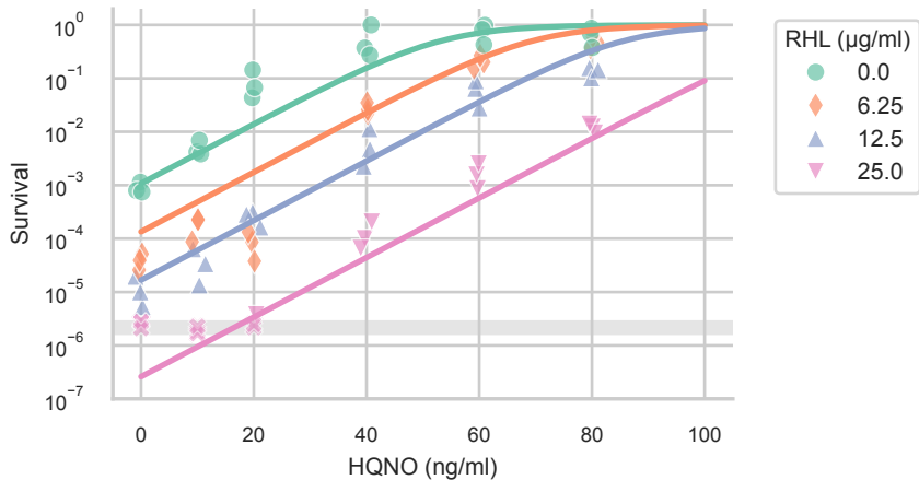
Linear Logit Model in RHL and HQNO (max HQNO: 80 ng/ml)
