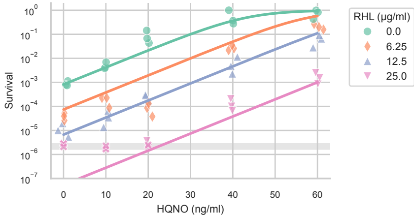
Linear Logit Model in RHL and HQNO (max HQNO: 60 ng/ml)
