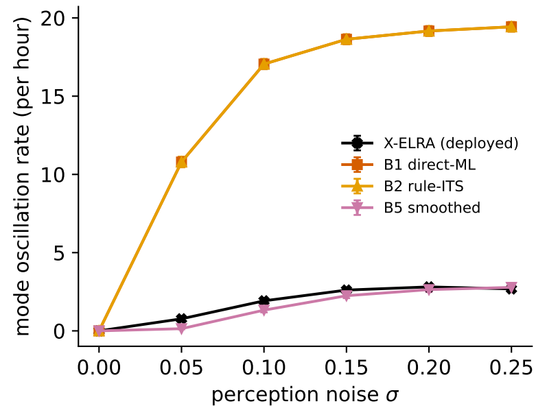
(a) Oscillation
