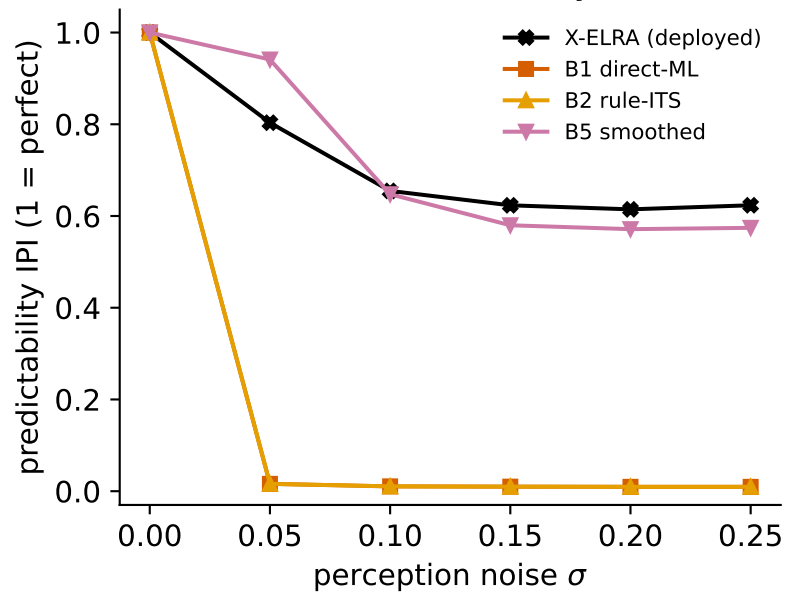
(b) Predictability
