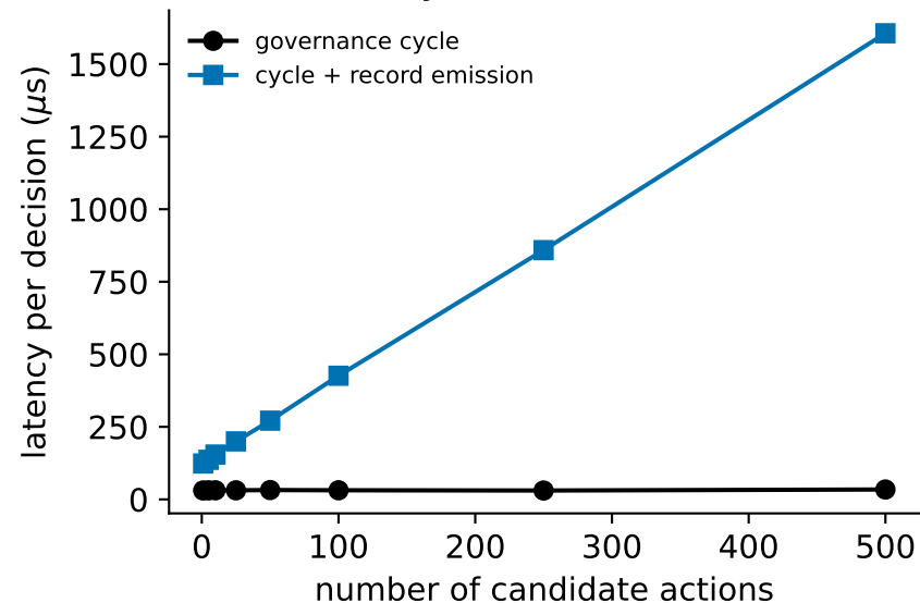
(a) Latency vs candidate-set size
