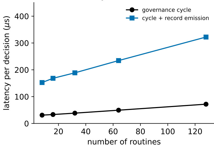
(b) Latency vs routine-set size
