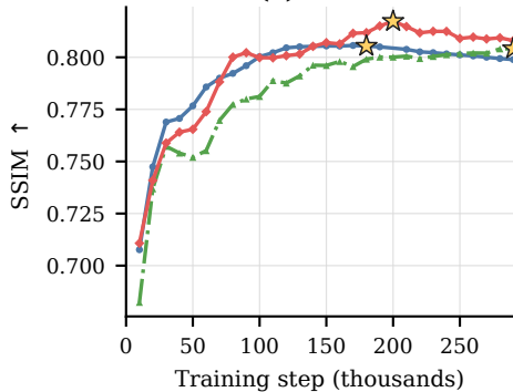
(a) SSIM
