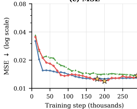
(c) MSE
