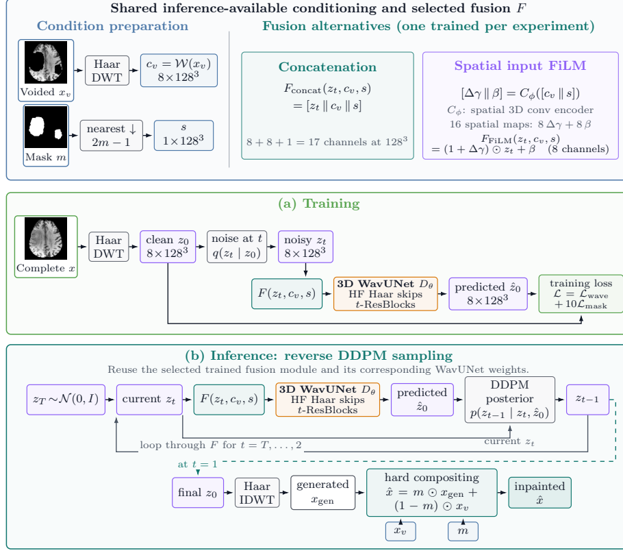
Fig. 1. Overview of CATCH. The voided image and downsampled signed mask are the only inference-time conditions. The framework supports either channel concatenation or spatial input FiLM. During training, the WavUNet predicts clean Haar coefficients and is supervised by the tumor-excluded wavelet loss and healthy-hole-focused mask loss. During inference, the current latent z_t and clean prediction \hat{z}_0 enter the DDPM posterior separately, and z_{t-1} returns through the selected fusion module. The final sampled z_0 is decoded into the output volume, after which hard compositing preserves x_v outside m exactly. The thumbnails show a geometry-selected training case on its maximum-mask-area axial slice; they are illustrative and were not selected using reconstruction performance.
