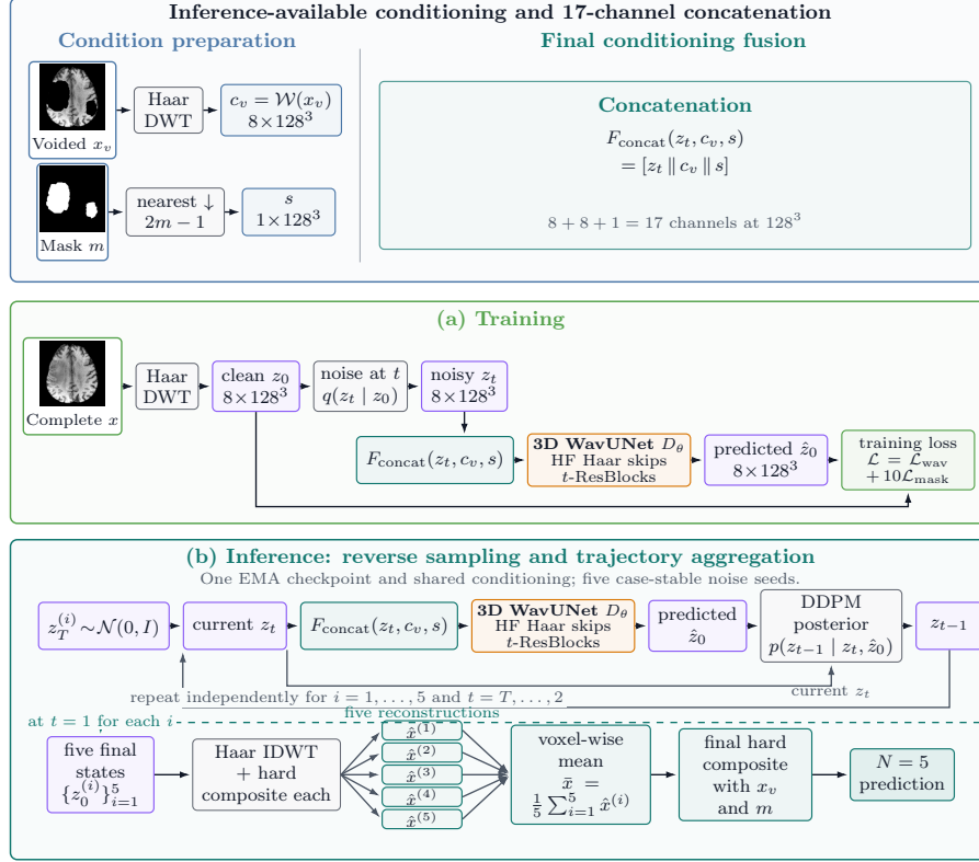
Fig. 1. CATCH training and inference. A Haar transform maps the voided image to eight subbands, concatenated with noisy target subbands and a signed mask. WavUNet predicts clean coefficients; inverse transformation and hard compositing restore the observed region. For selected random and weighted models, five case-stable noise seeds traverse one EMA checkpoint; their reconstructions are averaged voxel-wise and composited again. Fixed mask uses N = 1 . Input thumbnails were selected without reconstruction metrics.
