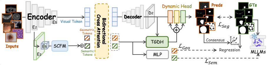
Token-Guided Dynamic Head (TGDH)
