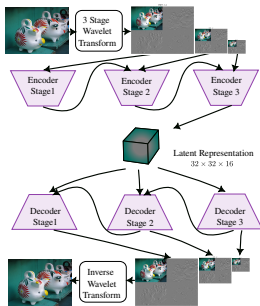
WF-VAE
