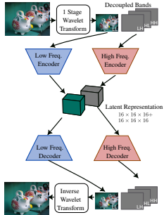
DeBaT (ours)
