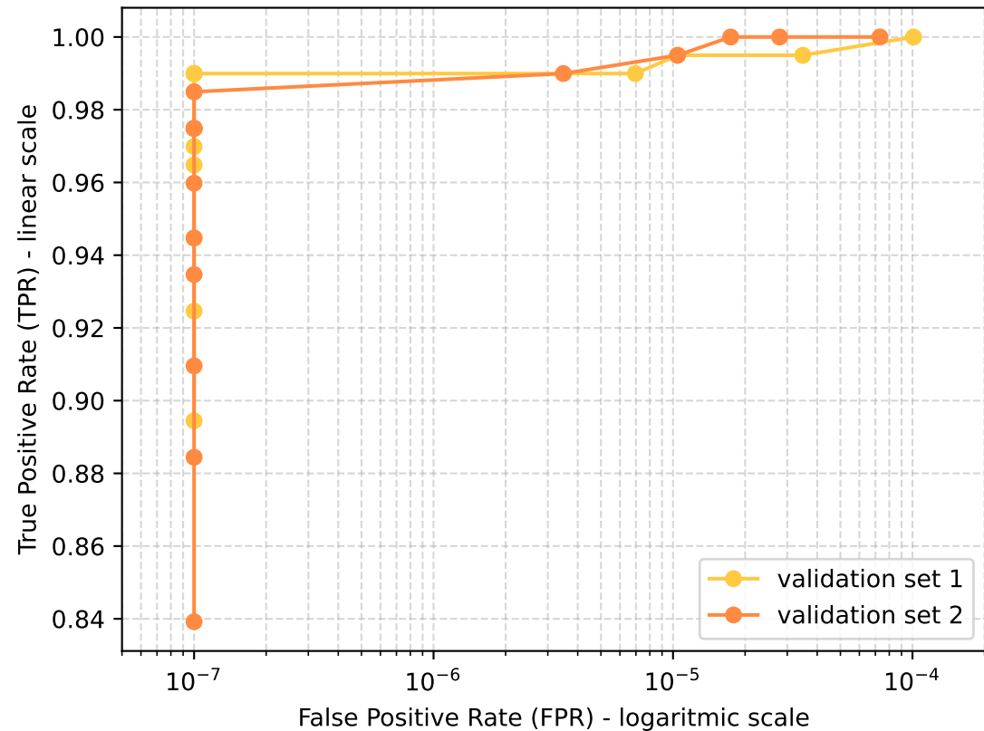
Semi Logarithmic ROC curve
