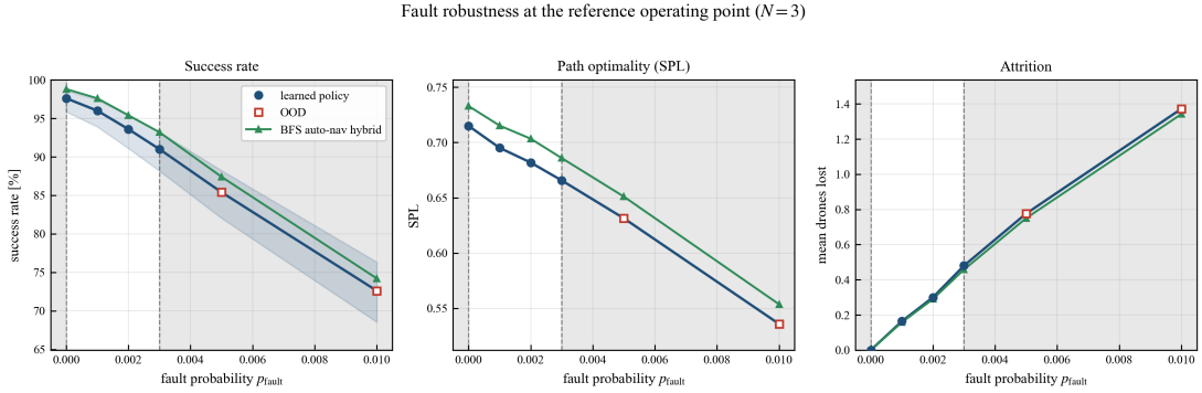
Figure 10: Fault robustness. Learned policy (blue) versus the BFS auto-nav hybrid (green); the shaded region is OOD ( p_{\text{fault}} > 0.003 ). Panels: success, SPL and the mean number of drones lost per episode.
