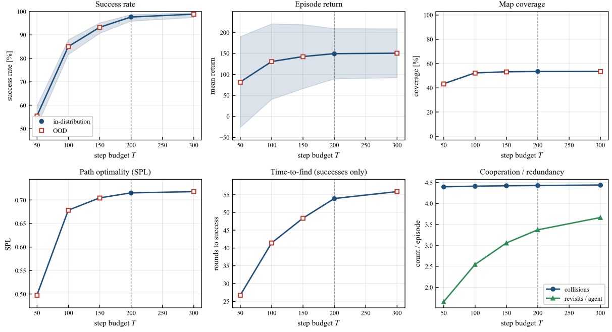
Figure 14: Sensitivity to the step budget T . Success rises with diminishing returns as the budget grows; a larger budget only rescues episodes that were already close to succeeding. The budget was never randomized, training having fixed T = 200 : the dashed line marks that single trained value, and every other point is an extrapolation, so the white/shaded convention of Section 7 does not apply on this axis.
