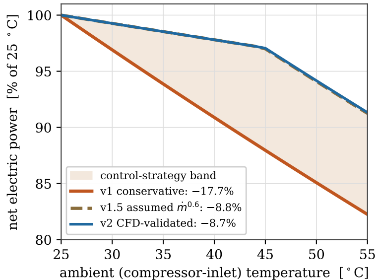
(a) the derating curve, three model generations
