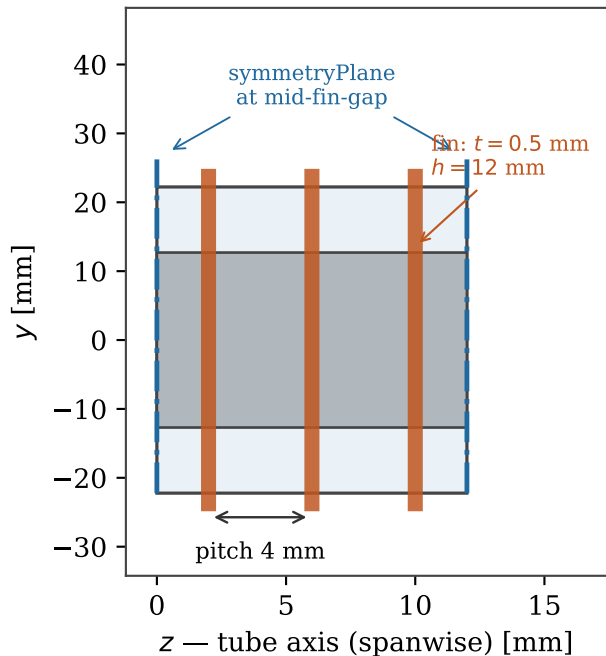
(b) 3-fin unit cell, y - z plane
