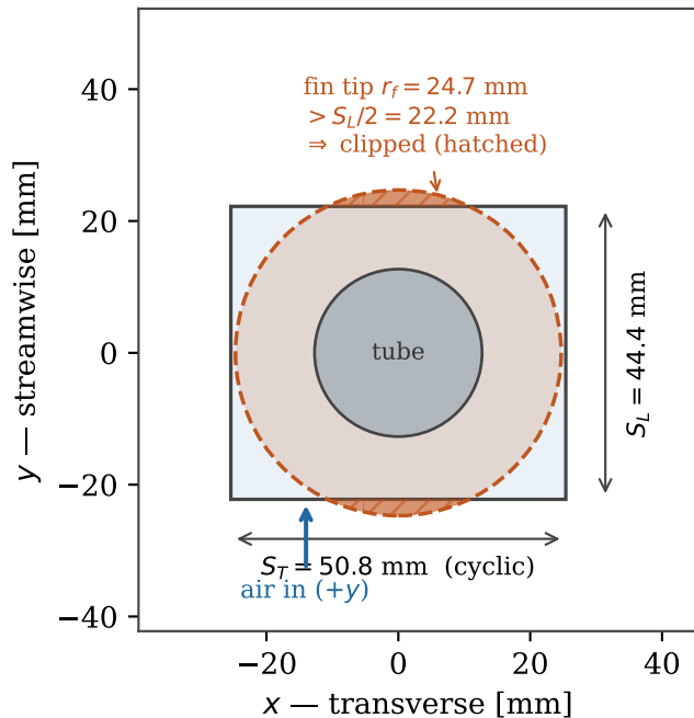
(a) unit cell, x - y plane
