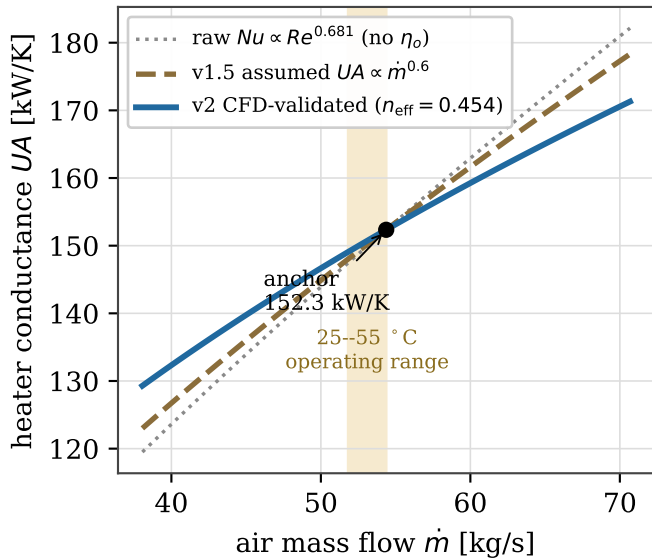
(a) the injected UA(\dot{m}) law
