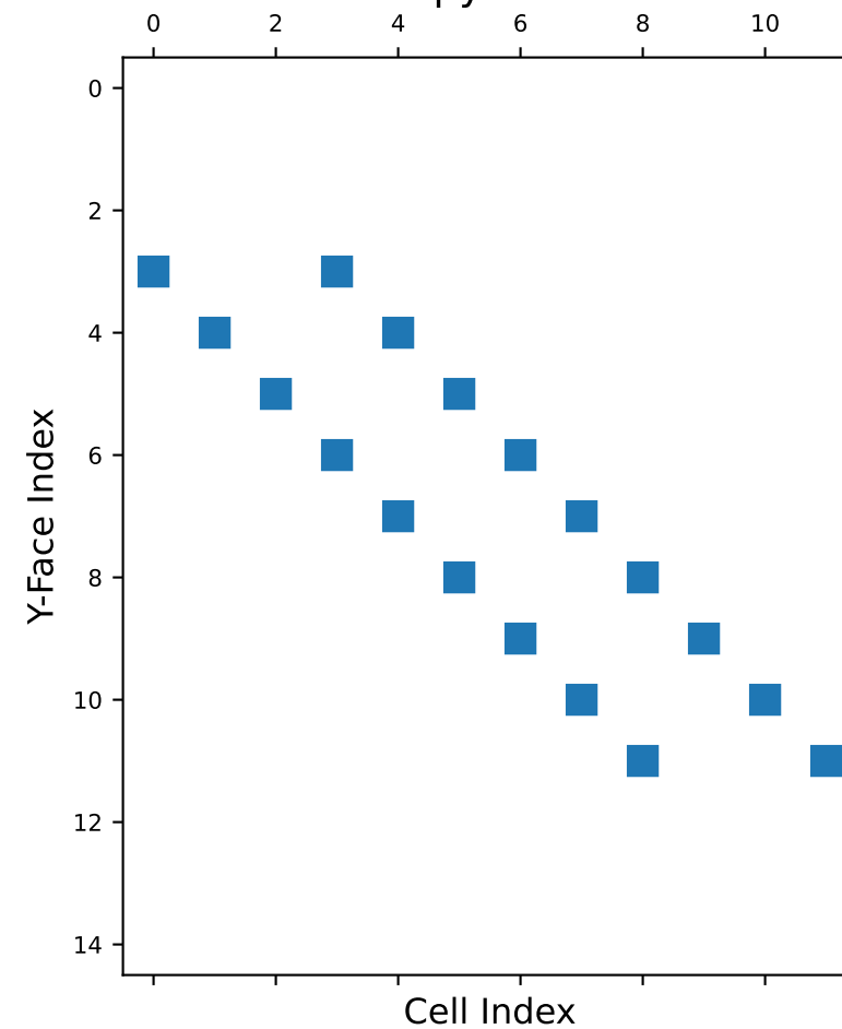
Spy Plot
