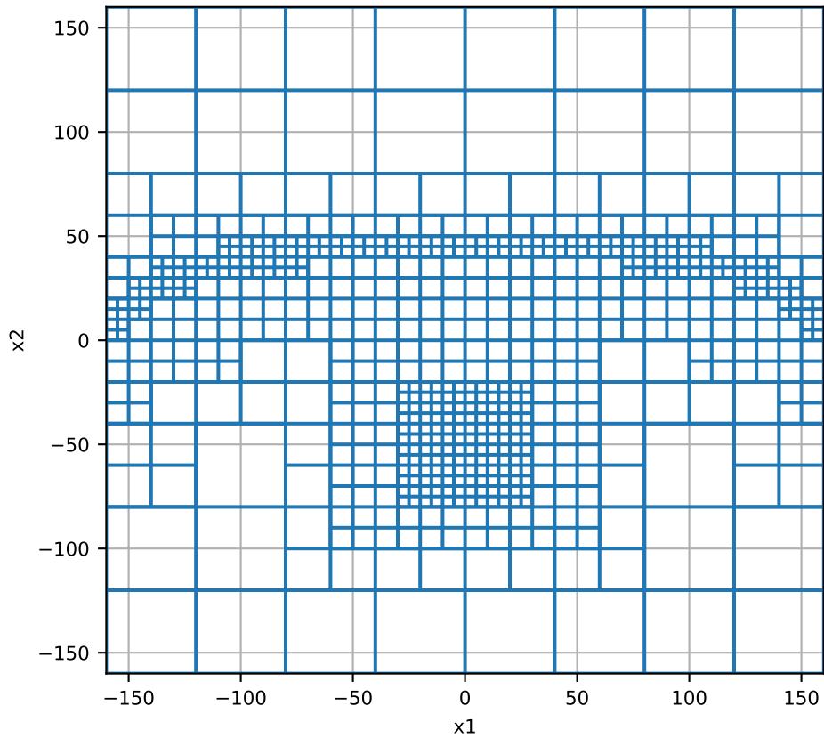
QuadTree Mesh
