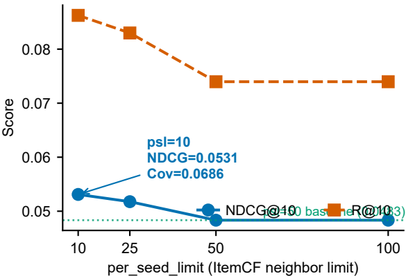
(b) ItemCF per_seed_limit vs NDCG@10 / R@10
