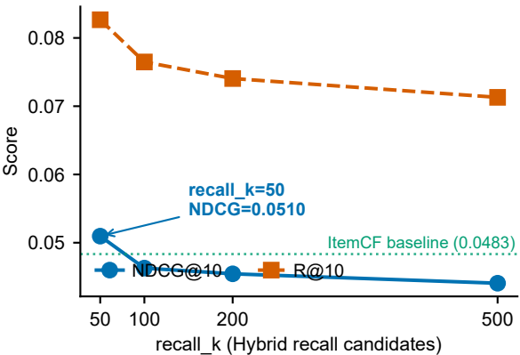
(a) Hybrid recall_k vs NDCG@10 / R@10
