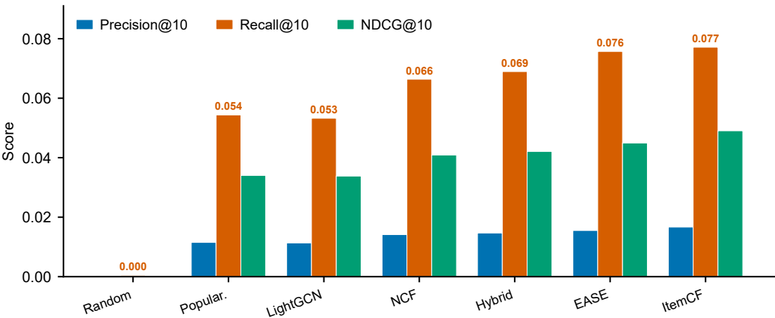
(a) C_all=13K protocol — 7 models, full ranking, 10K users
