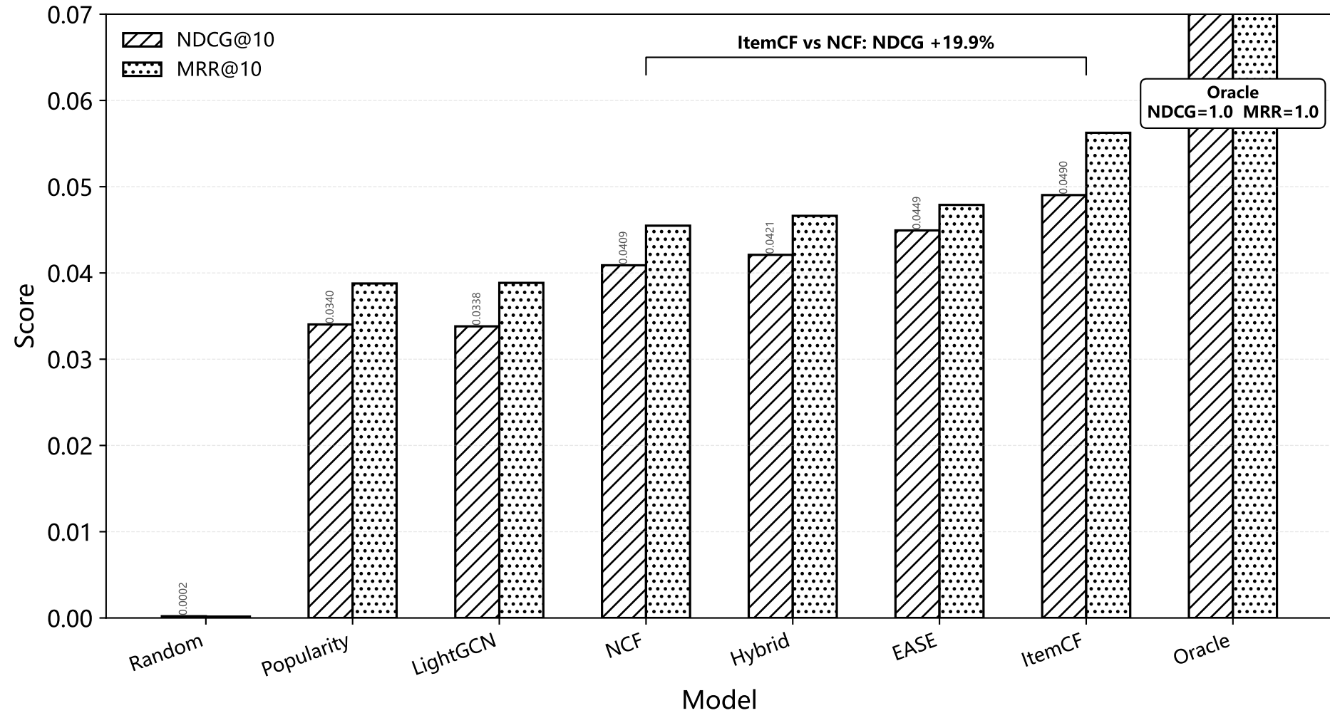
Model Ranking Quality Comparison (K=10, C_all=13304, 10k users)
