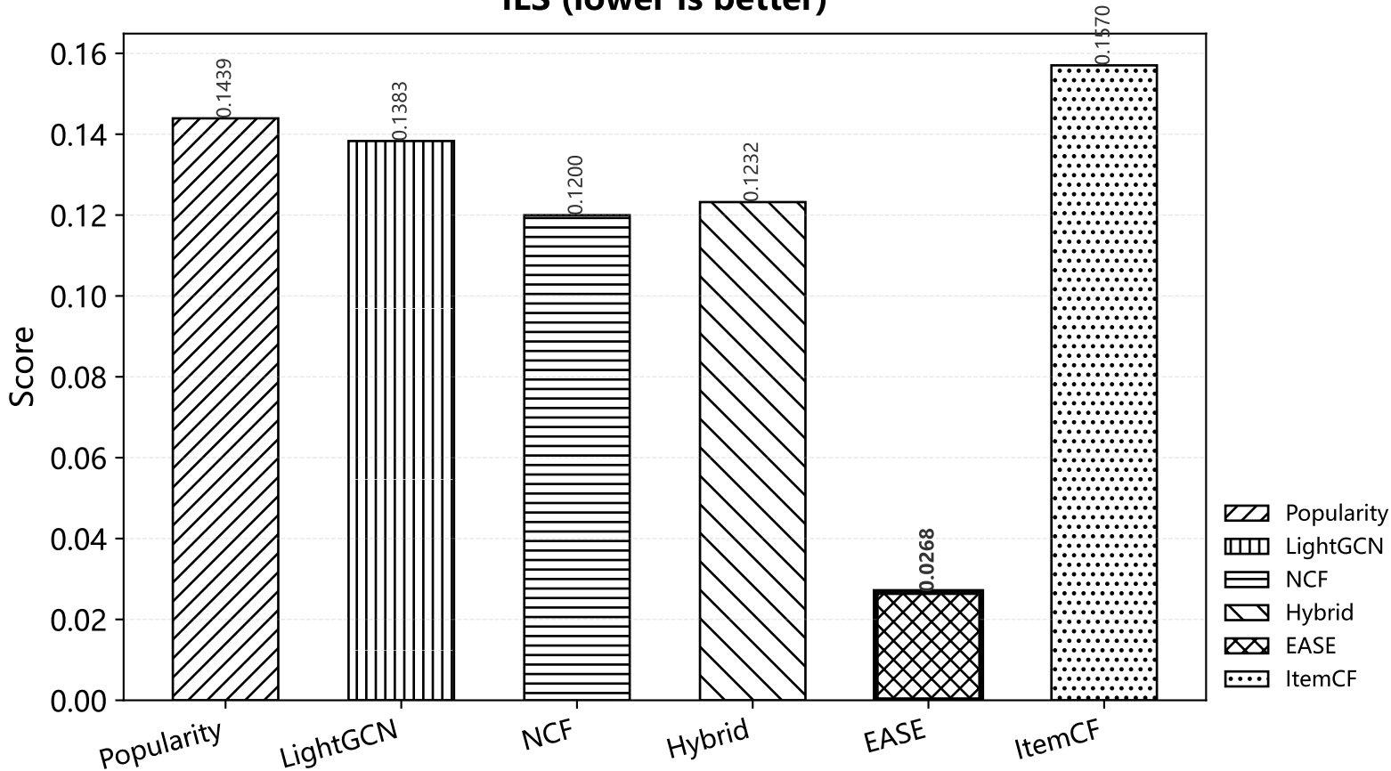
ILS (lower is better)
