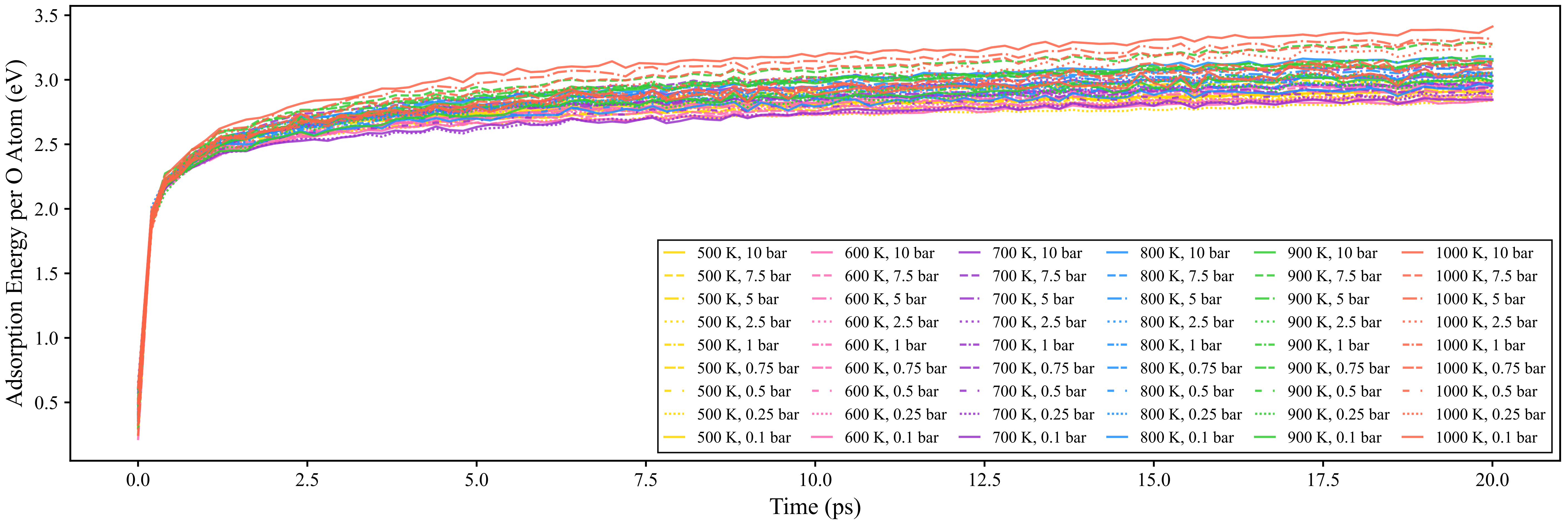
(a) Time vs Adsorption Energy per O Atom (Averaged)
