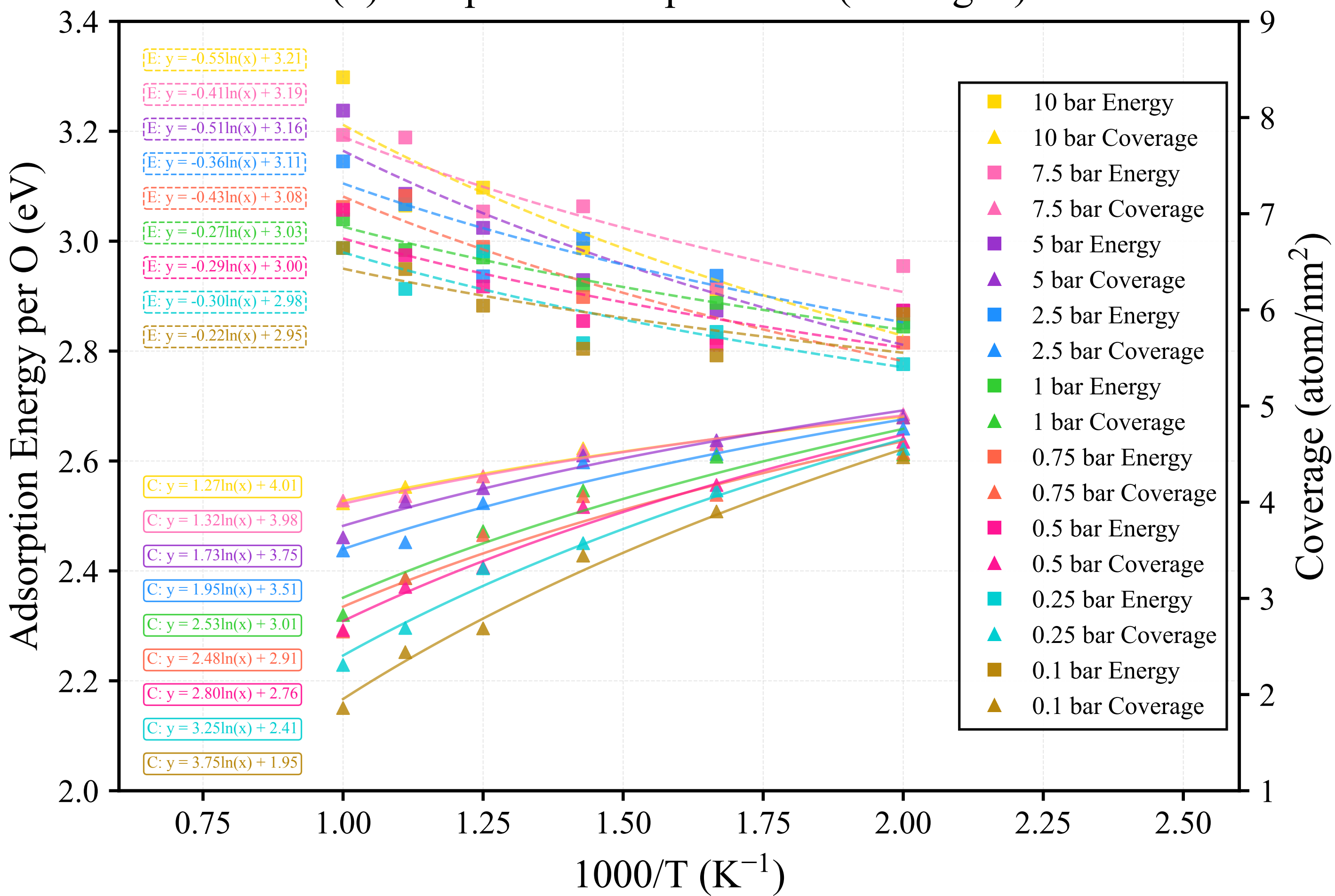
(b) Temperature Dependence (Averaged)
