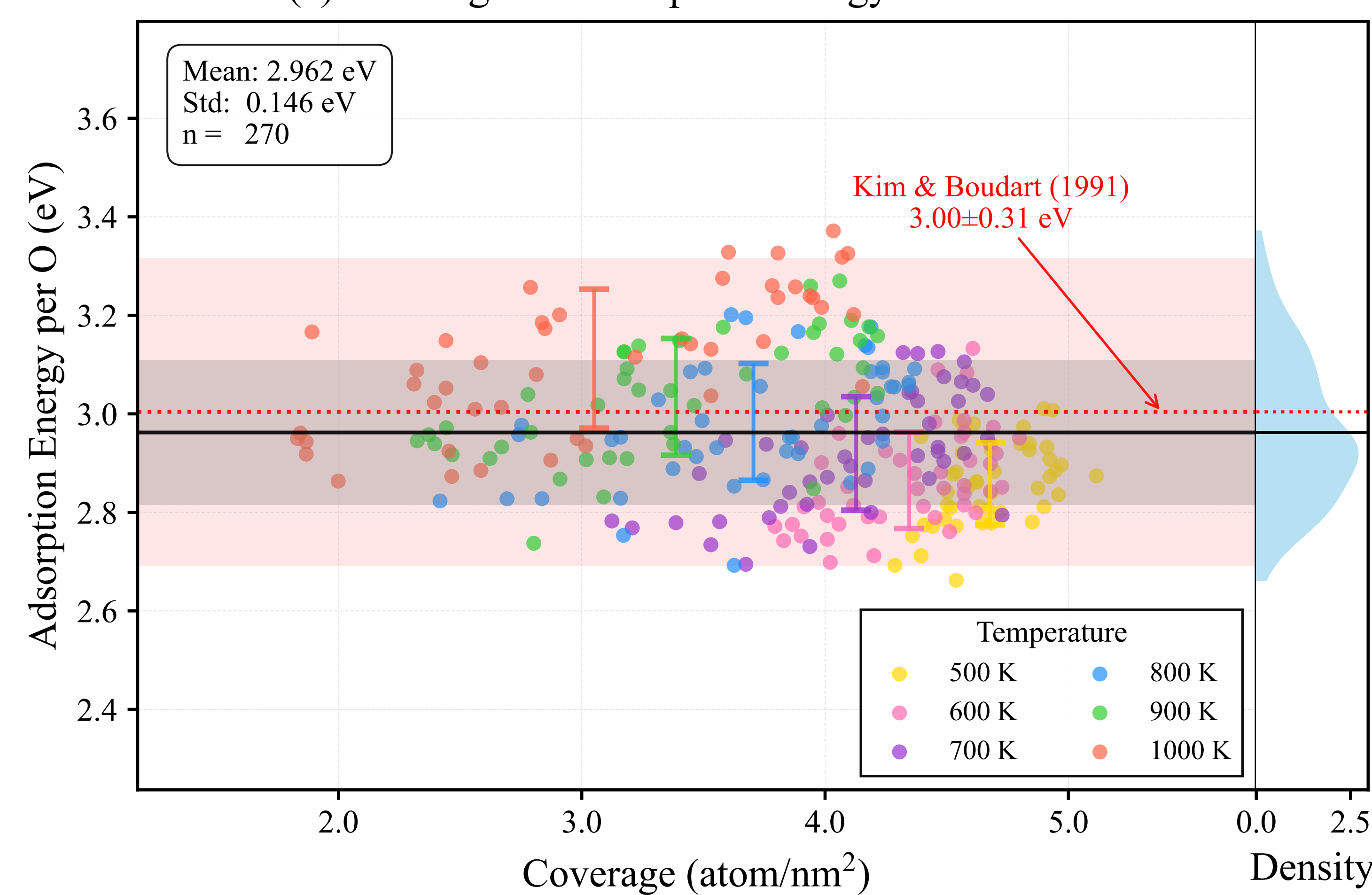
(c) Coverage vs Adsorption Energy Distribution
