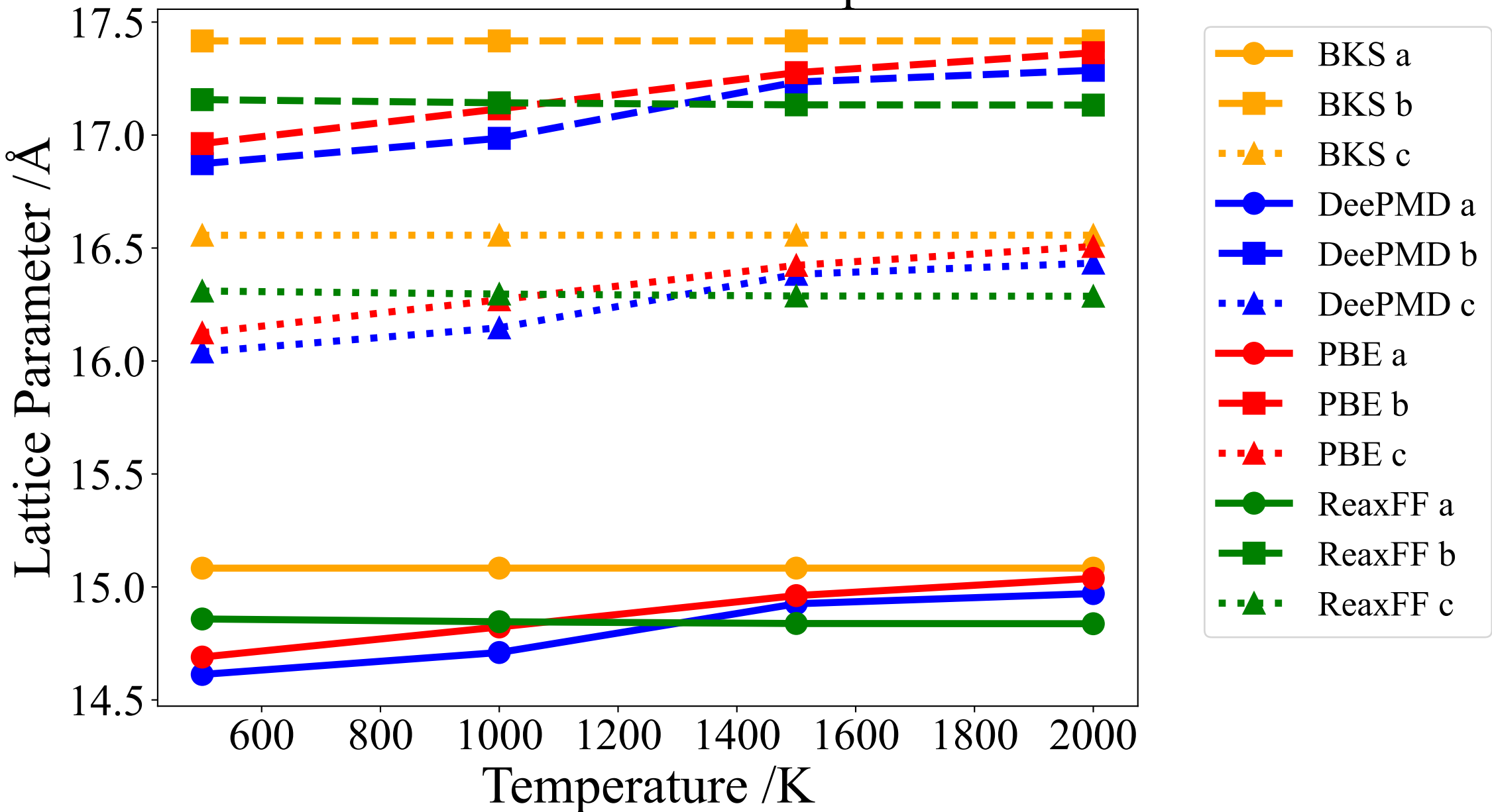
Lattice Parameters vs Temperature
