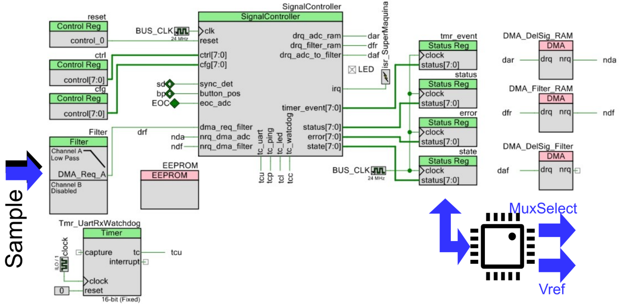
Fig. 3: Core PSoC digital hardware implementing the calibration workflow: signal controller, programmable digital filter, DMA channels, status registers, and EEPROM record.
