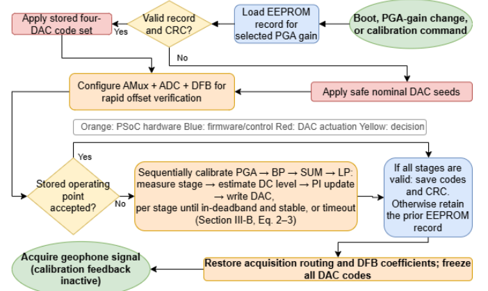
Fig. 1: Foreground calibration flow: stored-code verification, sequential trimming, and acquisition.
