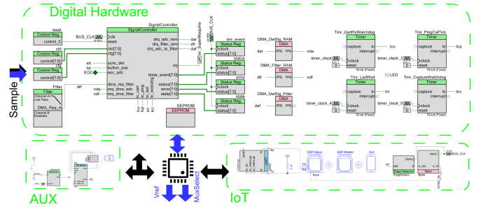
Fig. 3: Digital hardware implementing the calibration workflow (top); AUX/IoT blocks (bottom) belong to the broader platform [7], outside this paper's scope.
