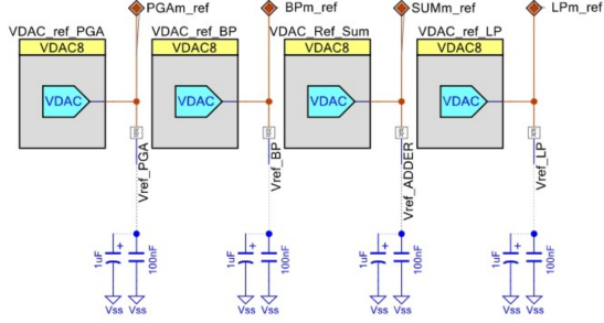
Fig. 1: Analog signal chain: four independent VDAC references trim the programmable-gain amplifier (PGA), band-pass filter (BP), summing stage (SUM), and low-pass filter (LP), with a shared ADC/multiplexer measurement path.
