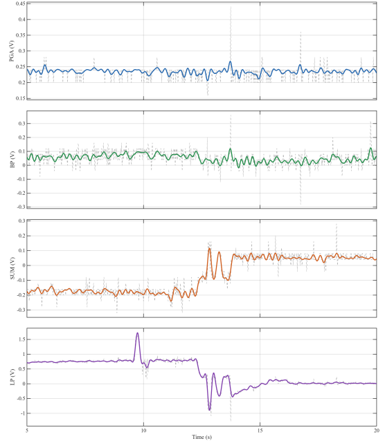
Fig. 4: Representative foreground calibration trajectories: stage deviations relative to V_{\text{ref}} during calibration at \times 16 gain (total differential gain \times 32 ). Dashed light-gray traces are oscilloscope measurements; colored curves are resampled 128-tap-FIR reconstructions, not internal logs (Section V).
