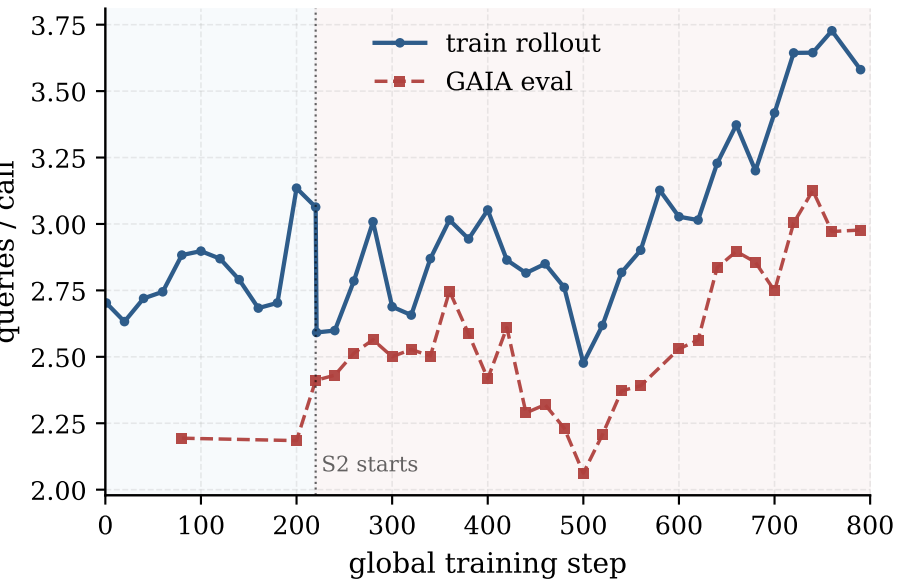
(g) Queries per search call
