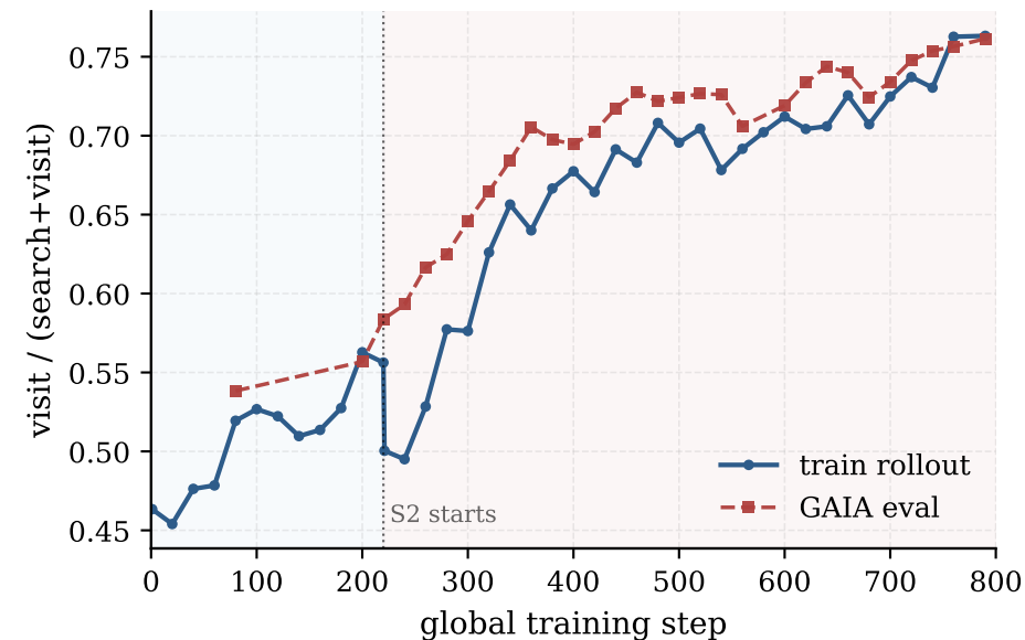
(f) Browse share of tool use
