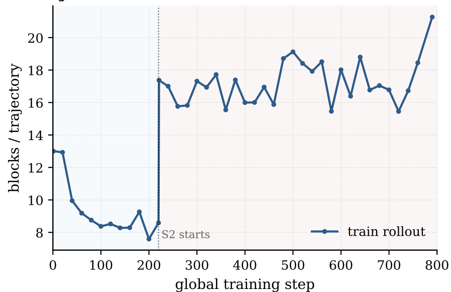
(j) # <think> blocks
