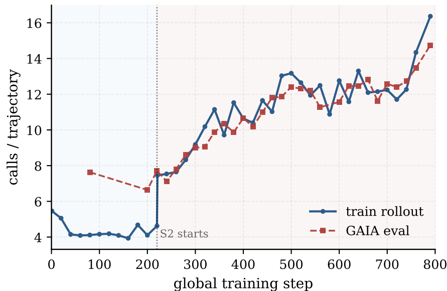
(e) Browse / visit calls
