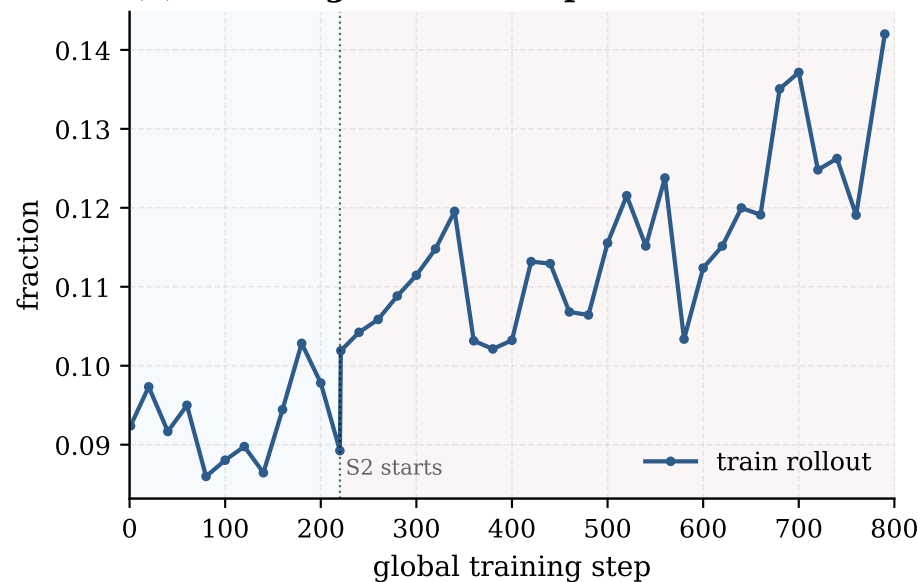
(k) Thinking share of output
