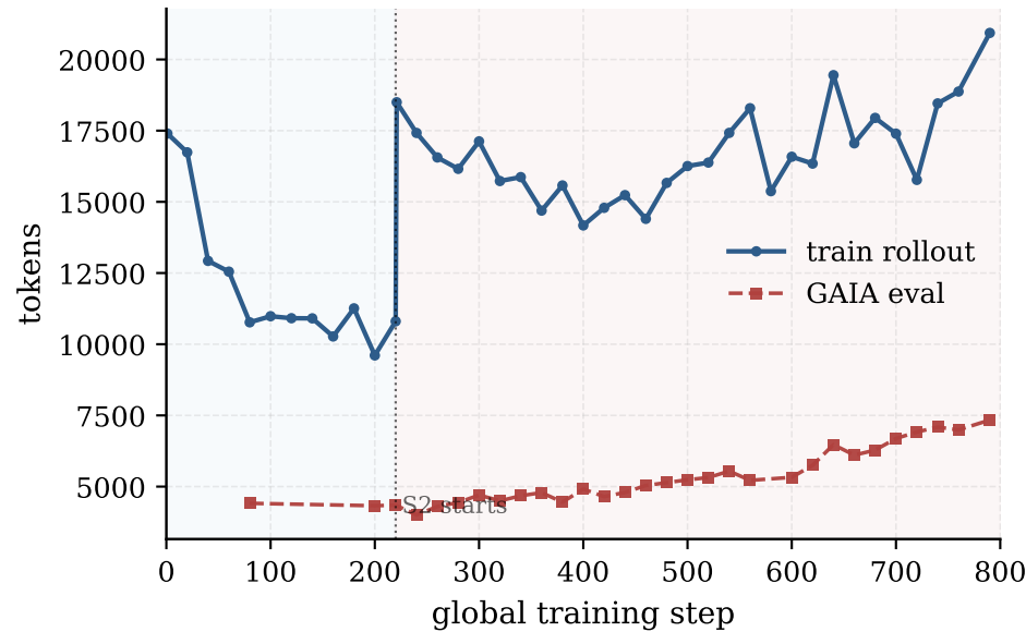
(b) Mean response length
