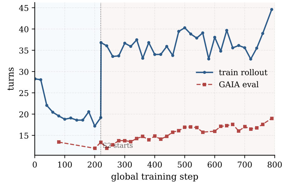
(c) # agent turns
