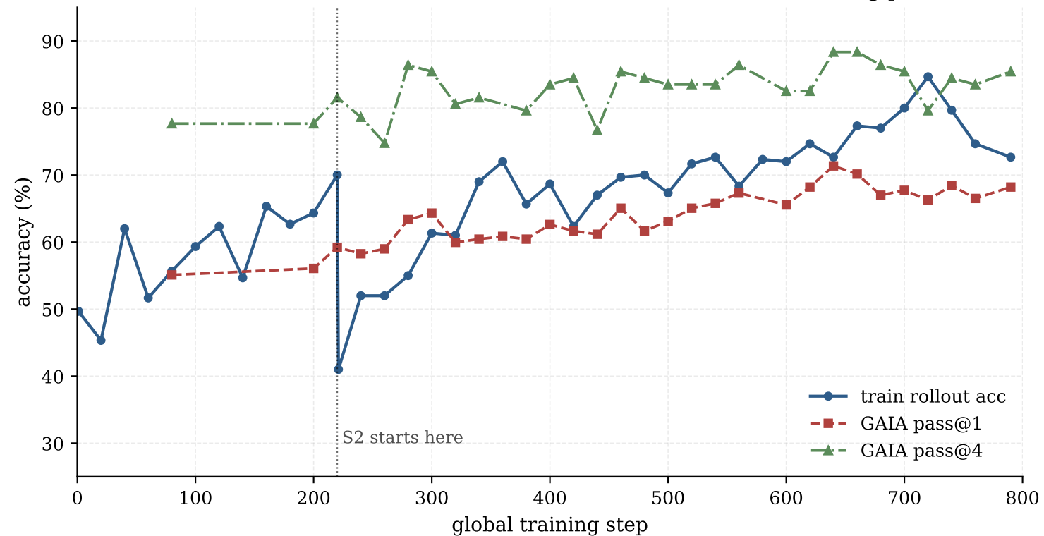
Train reward and GAIA evaluation across the continuous training path
