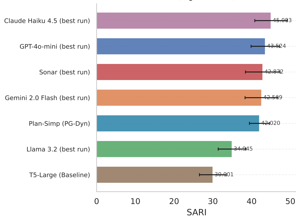
SARI (higher better)
