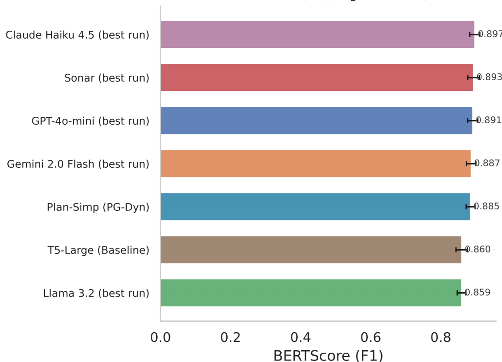
BERTScore (F1) (higher better)
