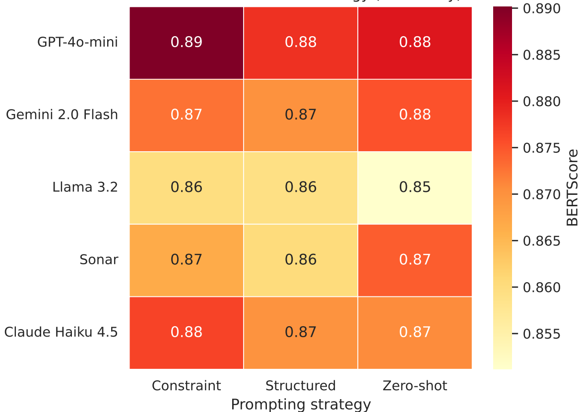
BERTScore — model × strategy (PE v2 only)
