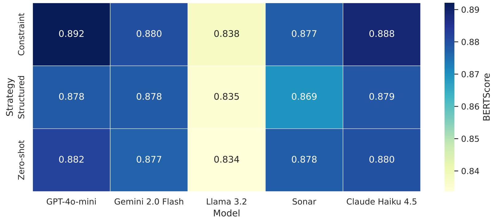
BERTScore — strategy × model (mean over all phases)
