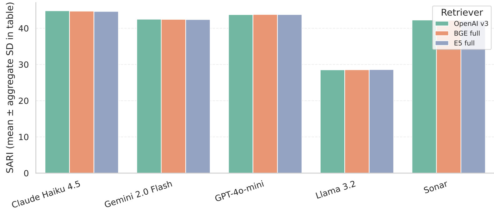
SARI by model and retriever — Constraint (RAG v3 / full)
