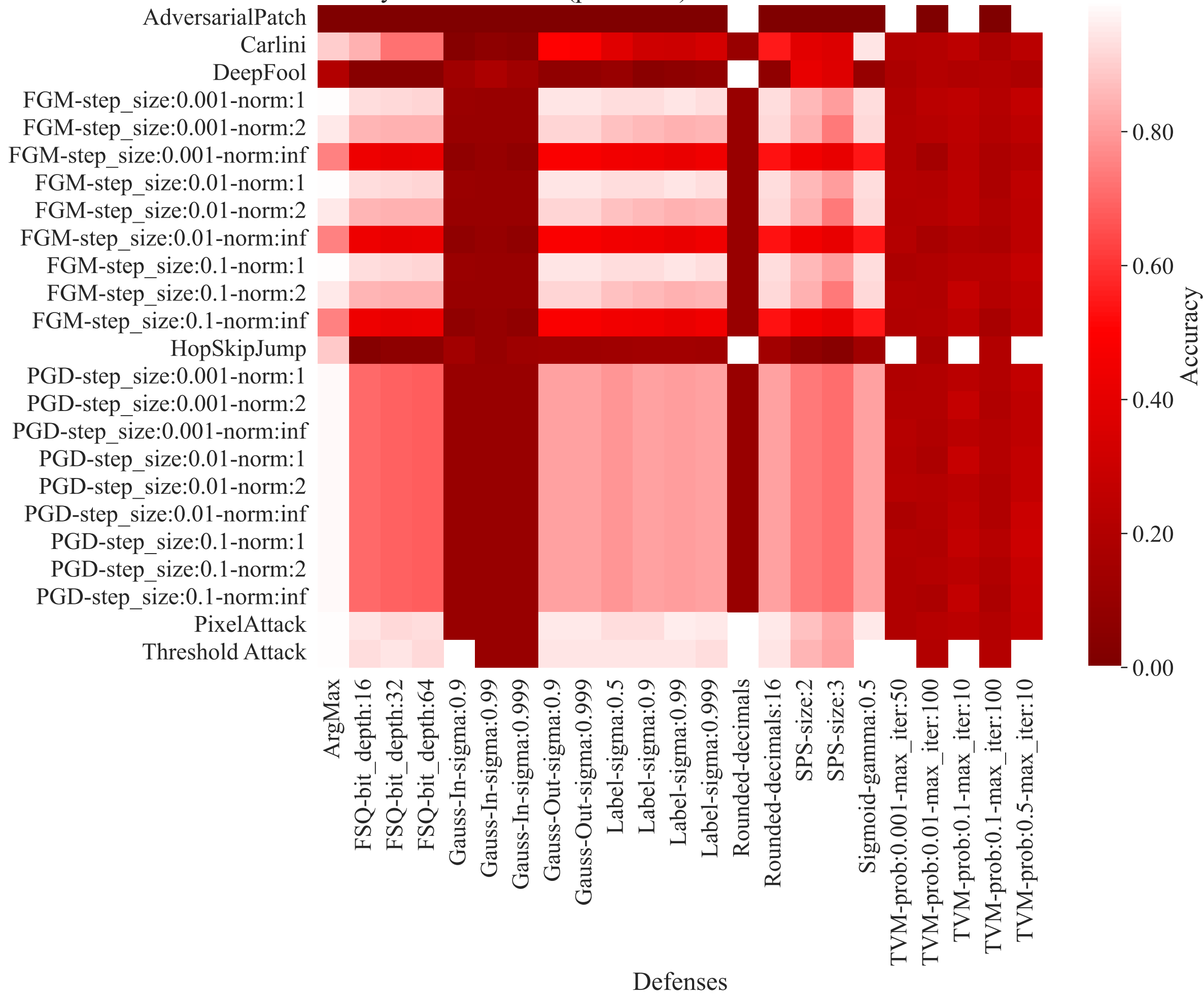
Accuracy on Adversarial (perturbed) data relative to undefended model.
