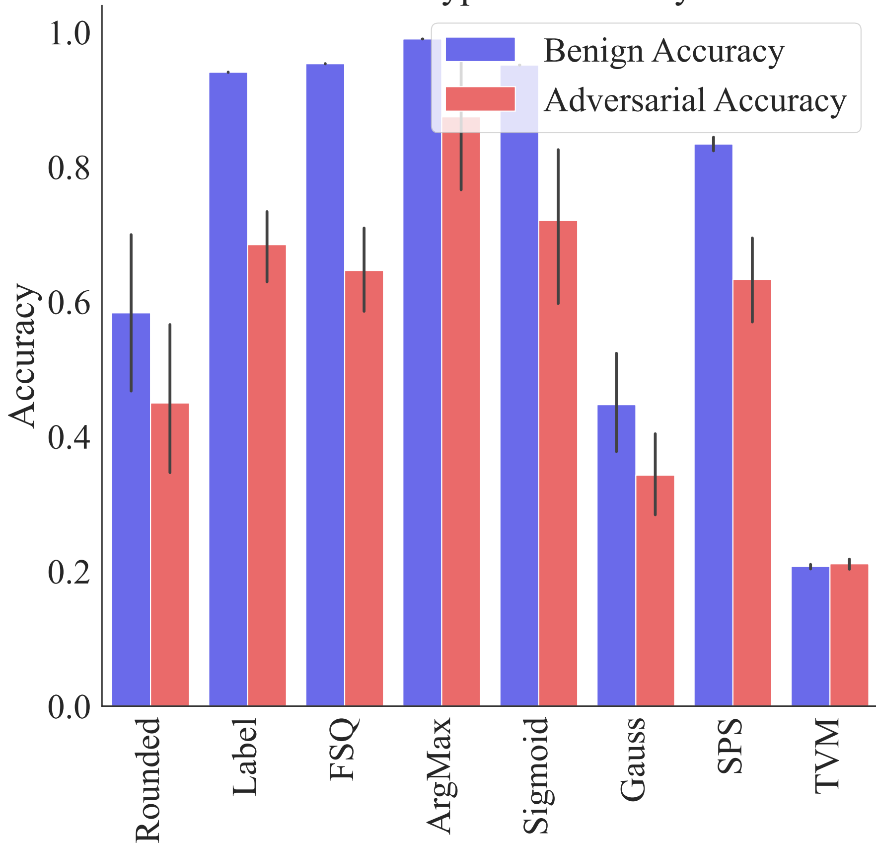
Defense Type vs Accuracy
