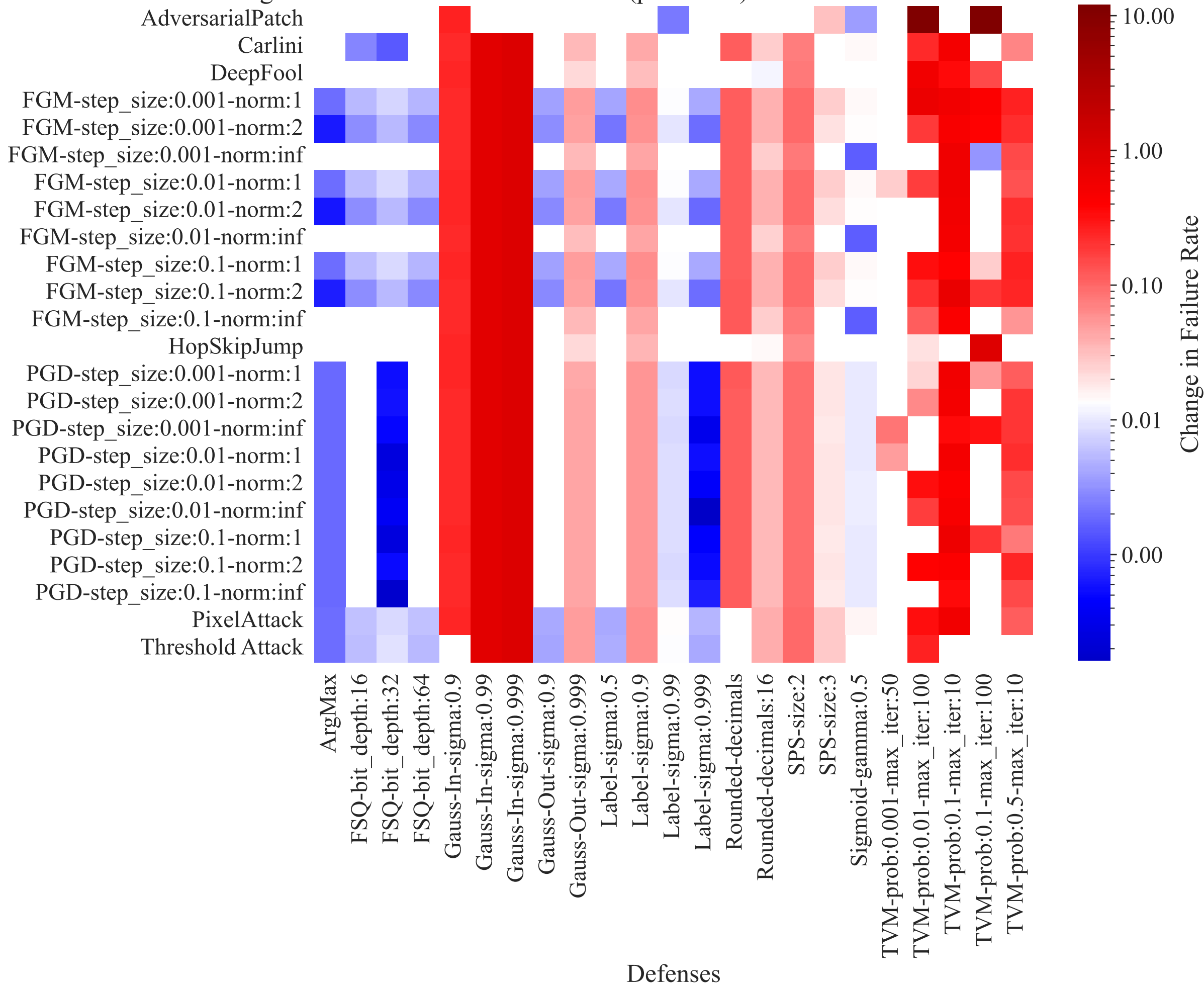
Change in Failure Rate On Adversarial (perturbed) Data Relative to Undefended Model
