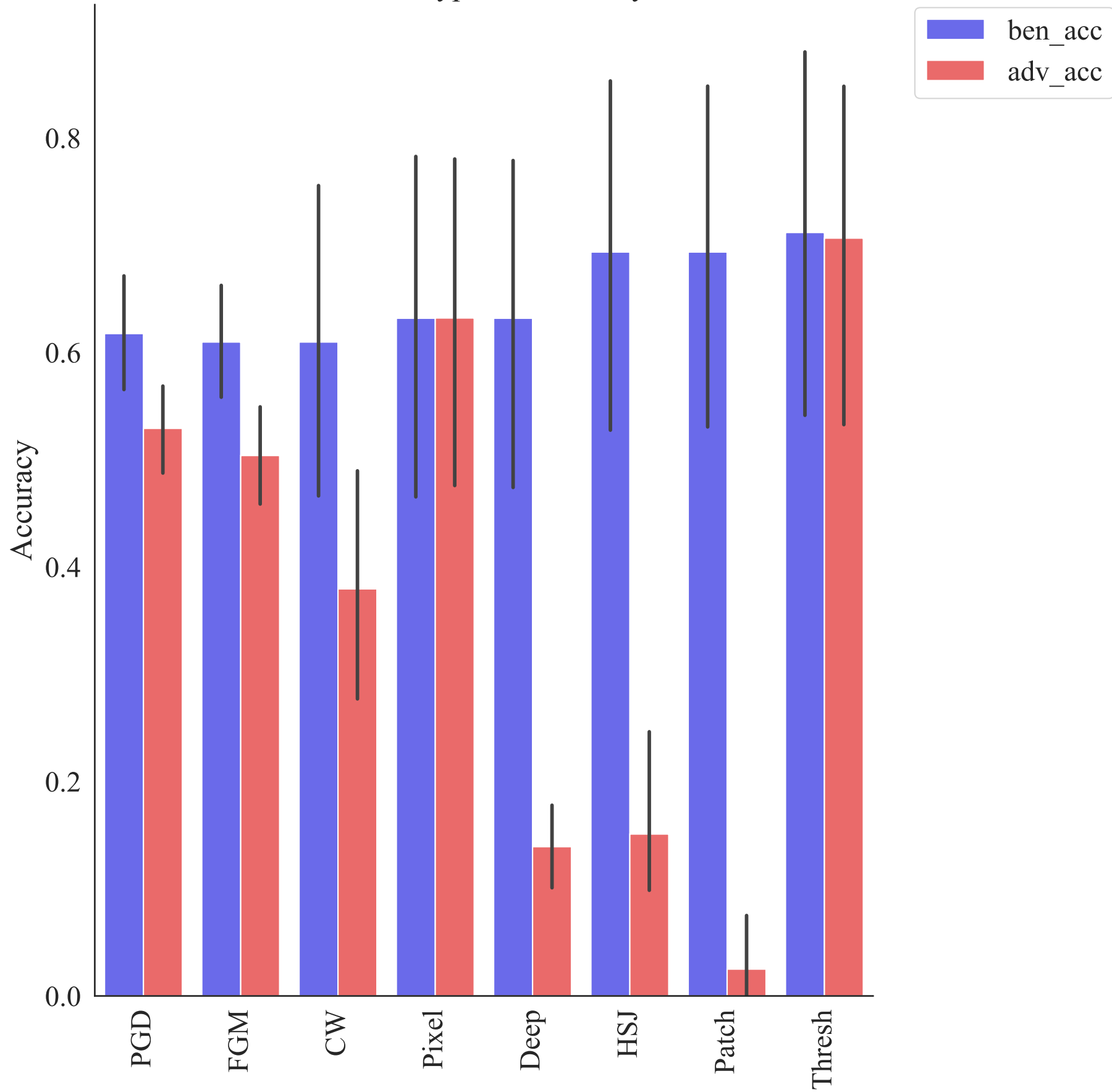
Attack Type vs Accuracy
