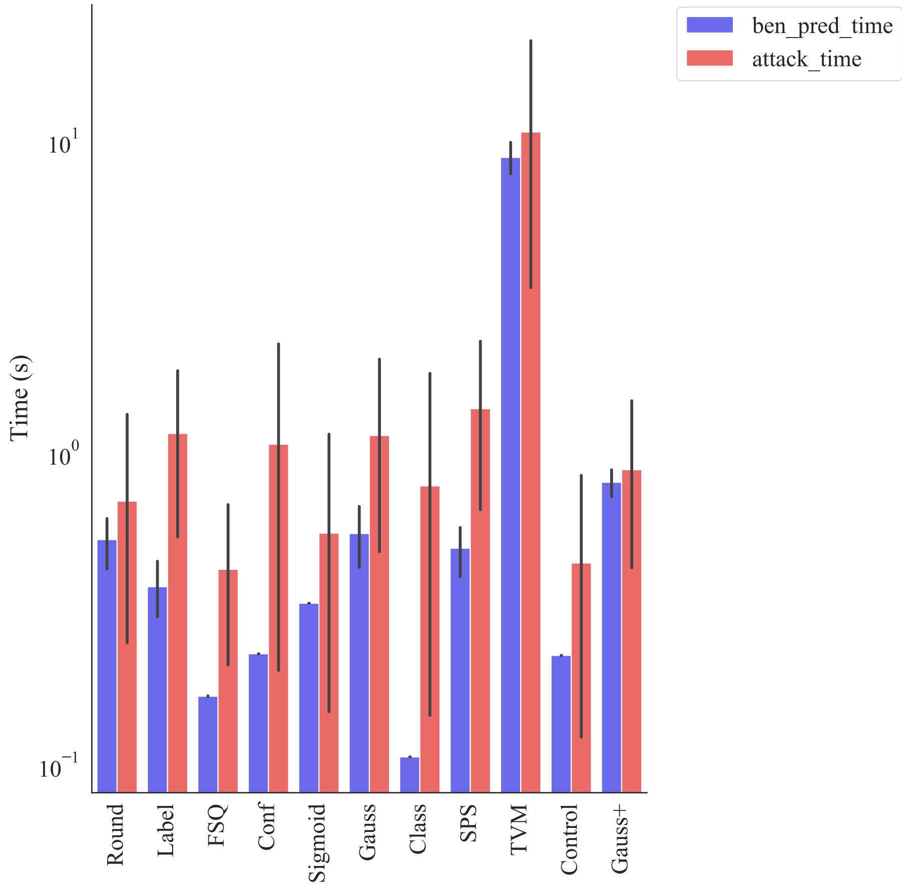
Normalized Prediction Time and Attack Time
