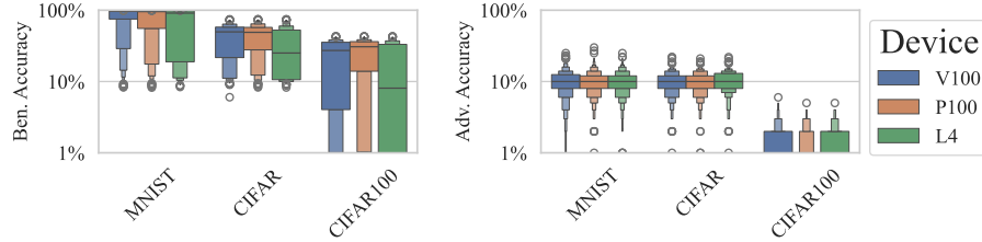
Fig. 3. Benign and adversarial accuracy across all hardware and datasets for all 1000 trials using plots that depict the distribution of the y-axis values using the width of the plot. Each colour is a different device and the datasets are displayed along the x-axis. Outliers are denoted with a white dot.
