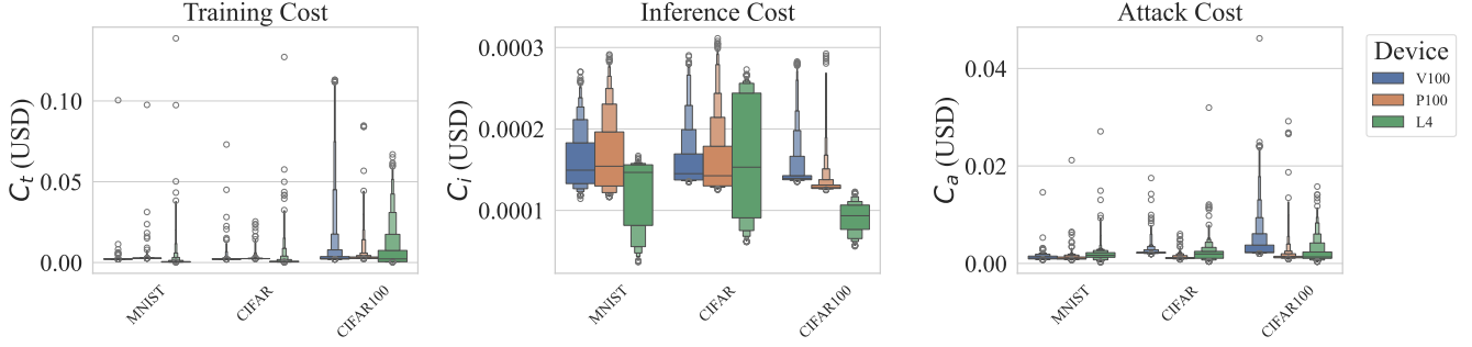
Fig. 5. This depicts the monetary cost during training, inference, and attack generation for all hardware and datasets for all 1000 trials using plots that depict the distribution of the second axis values using the width of the plot. The cost per sample was assumed to be uniform across the batch of samples for each training, inference, or attack measurement. Each colour is a different device and the datasets are displayed along the first axis. Outliers are denoted with a white dot. For these plots, the second axes have been scaled by the number of samples for the sake of comparison.
