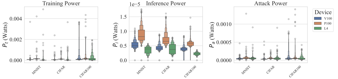
Fig. 4. This depicts the power consumption during training, inference, and attack generation for all hardware and datasets for all 1000 trials using plots that depict the distribution of the second axis values using the width of the plot. The power per sample was assumed to be uniform across the batch of samples for each training, inference, or attack measurement. Each colour is a different device and the datasets are displayed along the first axis. Outliers are denoted with a white dot. For these plots, the second axes have been scaled by the number of samples for the sake of comparison.
