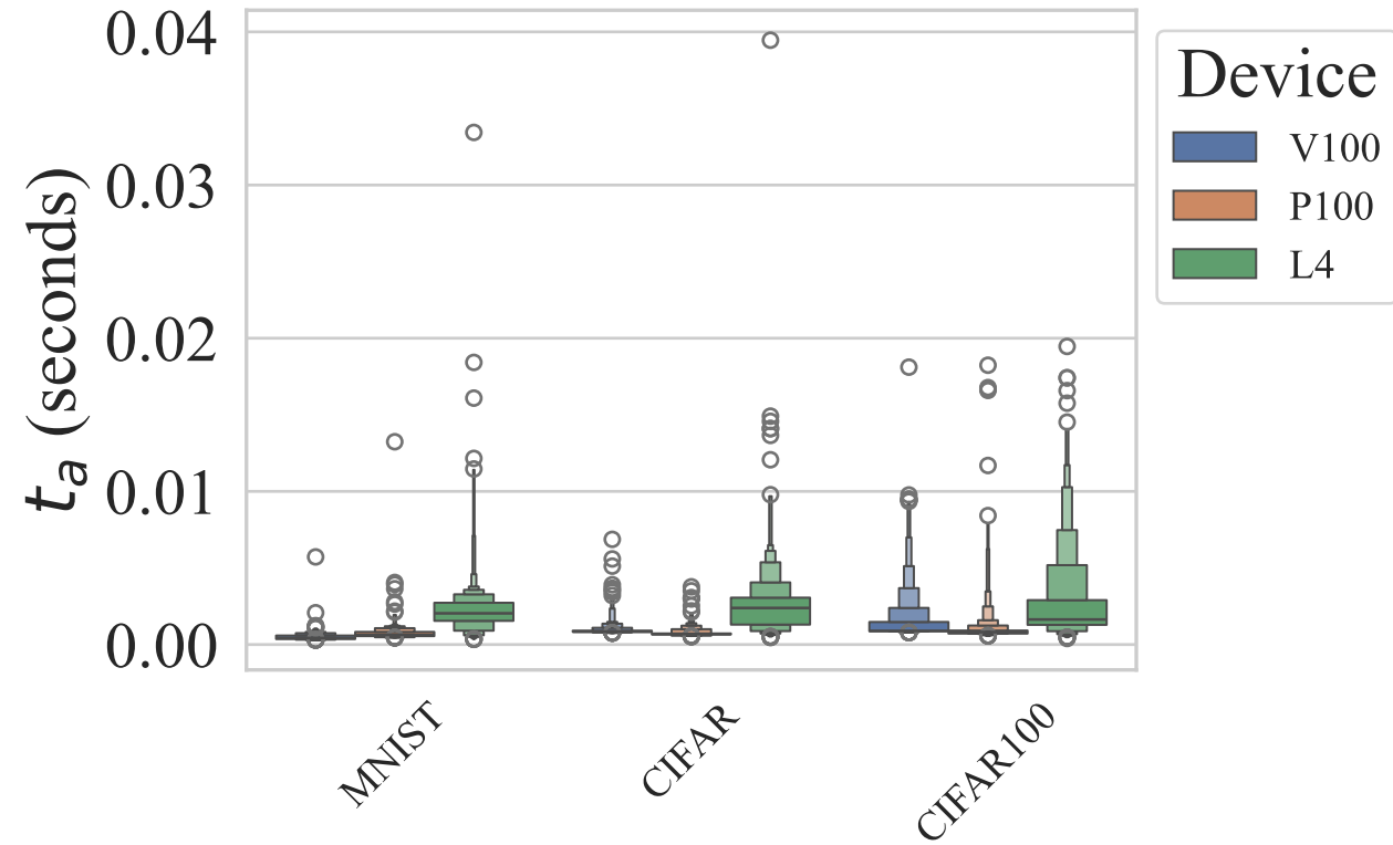
Attack Time
