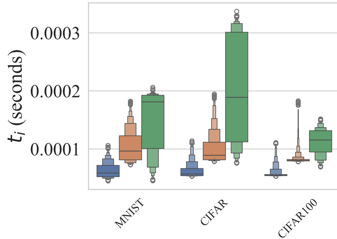
Inference Time
