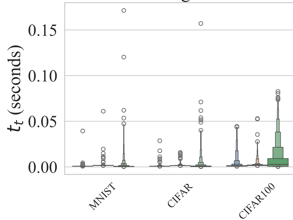
Training Time
