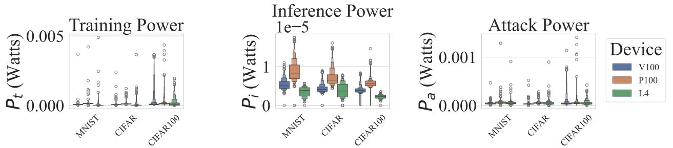
Fig. 4. Here we depict the power consumption during training, inference, and attack generation for all hardware and datasets for all 1,000 trials using plots that depict the distribution of the second axis values using the width of the plot. The power per sample was assumed to be uniform across the batch of samples for each training, inference, or attack measurement. Each colour is a different device and the datasets are displayed along the first axis. Outliers are denoted with a white dot. For these plots, the second axes have been scaled by the number of samples for the sake of comparison.
