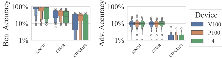
Fig. 3. Benign and adversarial accuracy across all hardware and datasets for all 1,000 trials using plots that depict the distribution of the first axis values using the width of the plot. Each colour is a different device and the datasets are displayed along the first axis. Outliers are denoted with a white dot.
