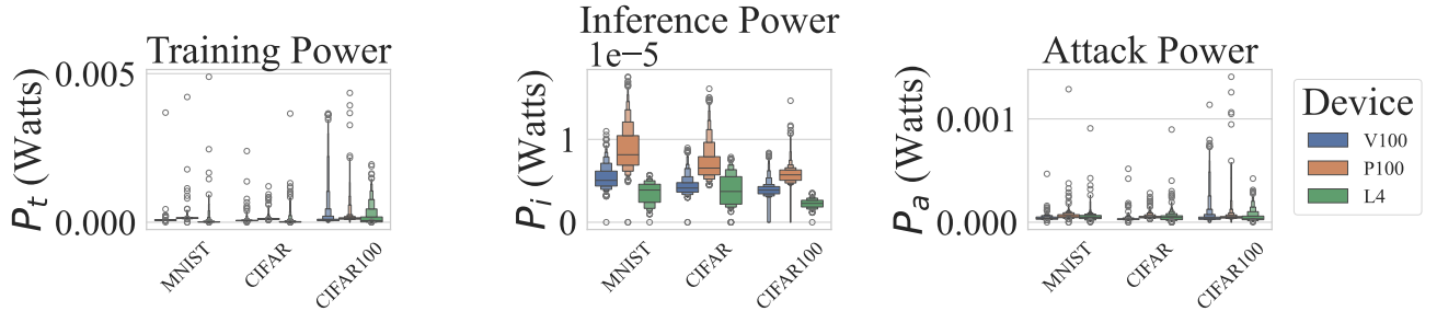
Fig. 4. Here we depict the power consumption during training, inference, and attack generation for all hardware and datasets for all 1,000 trials using plots that depict the distribution of the second axis values using the width of the plot. The power per sample was assumed to be uniform across the batch of samples for each training, inference, or attack measurement. Each colour is a different device and the datasets are displayed along the first axis. Outliers are denoted with a white dot. For these plots, the second axes have been scaled by the number of samples for the sake of comparison.
