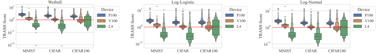
Fig. 5. The training rate and survival heuristic score (TRASH score) that depicts the per-sample ratio of training time to attack time for each of the tested AFT models. If this value is greater than one (the red line), then the model can be discarded as ineffective. The first axis shows each dataset, the second axis shows the TRASH score and each GPU model is given its own colour. Outlier scores are depicted with a white dot.
