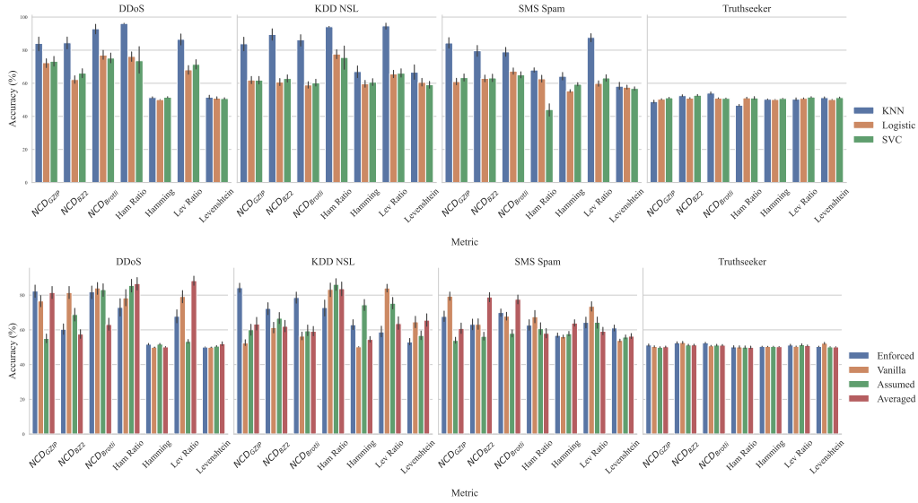
Figure 1: The accuracy across each dataset (columns), distance metric (first-axis), model (top plot, colour), and symmetrisation method (bottom plot, colour). For both plots, the bars represent the mean accuracy and the error bars represent 95% confidence intervals.
