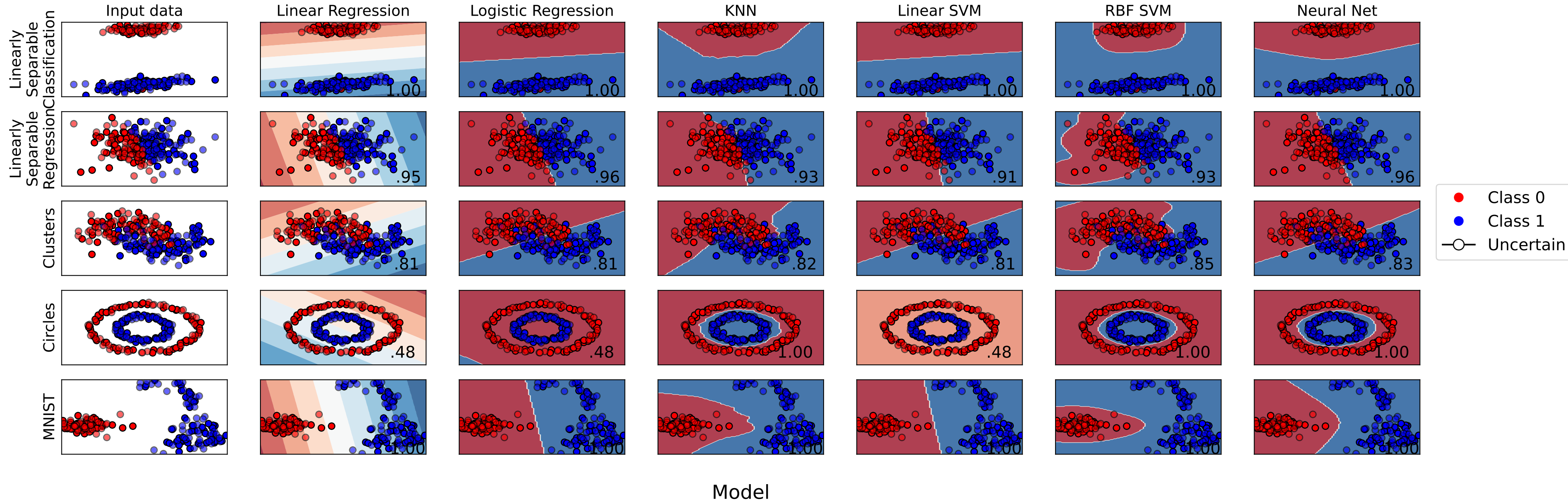
Classifiers Comparison
