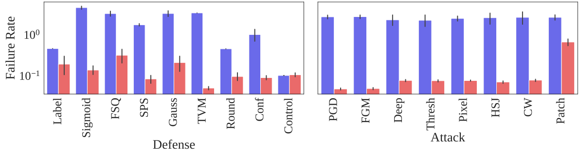
Fig. 14. The 95% confidence interval of failure rates both benign (blue) and adversarial (red) for CIFAR-10, broken down by defence (left) and attack (right). This was computed using Equation 2. The failure rate of the benign (unperturbed) dataset is depicted in blue and the failure rate of the adversarial (perturbed) dataset is depicted in red.
