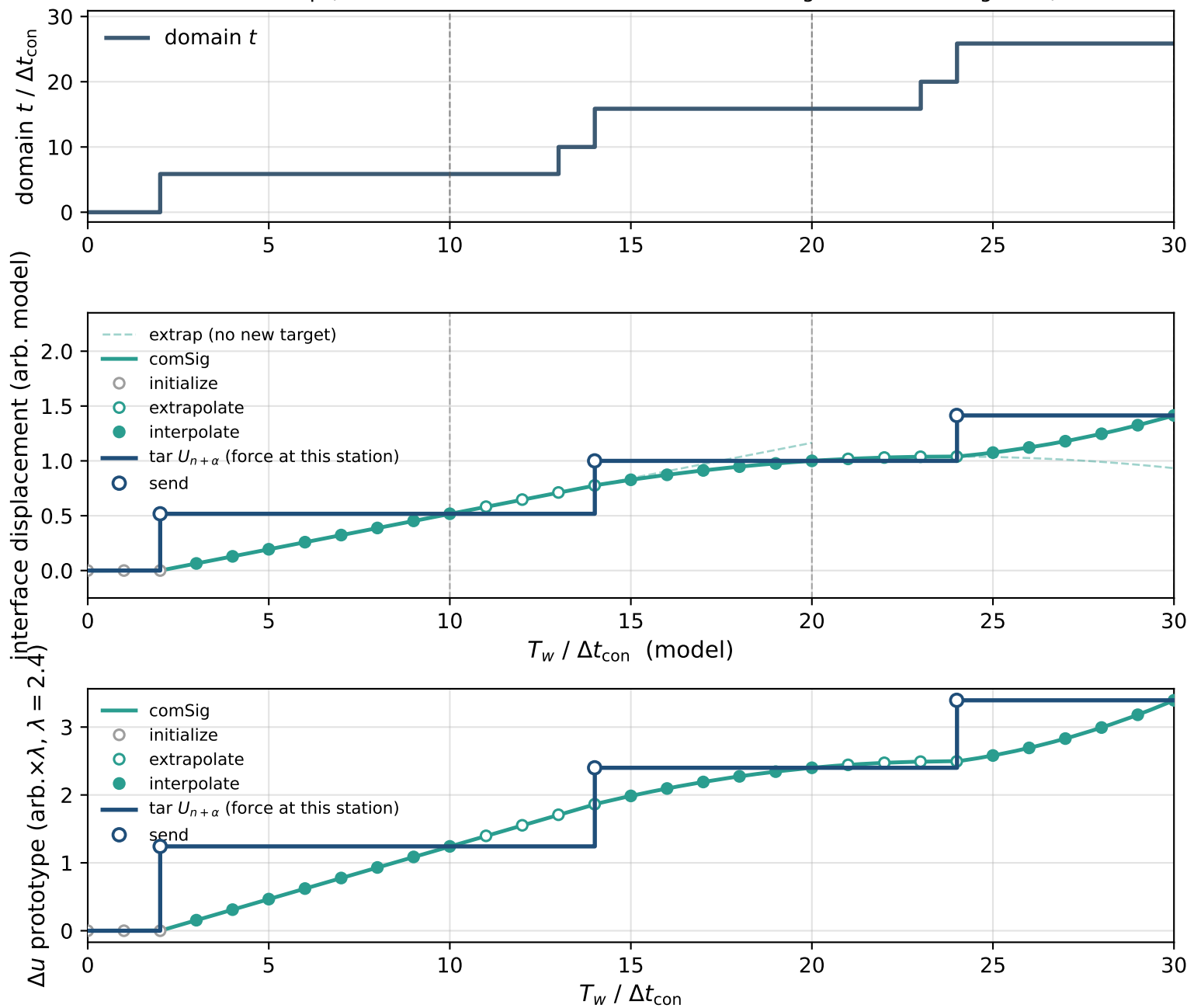
Three-window mockup (domain t at \alpha when force is read; tar / comSig; finish = 3 + begin = 1)
