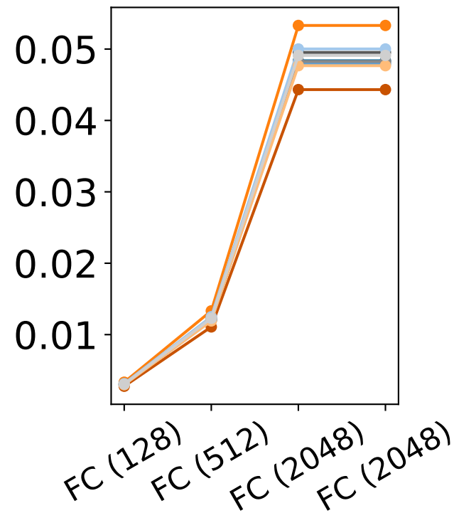
CNN-Fashion-MNIST
