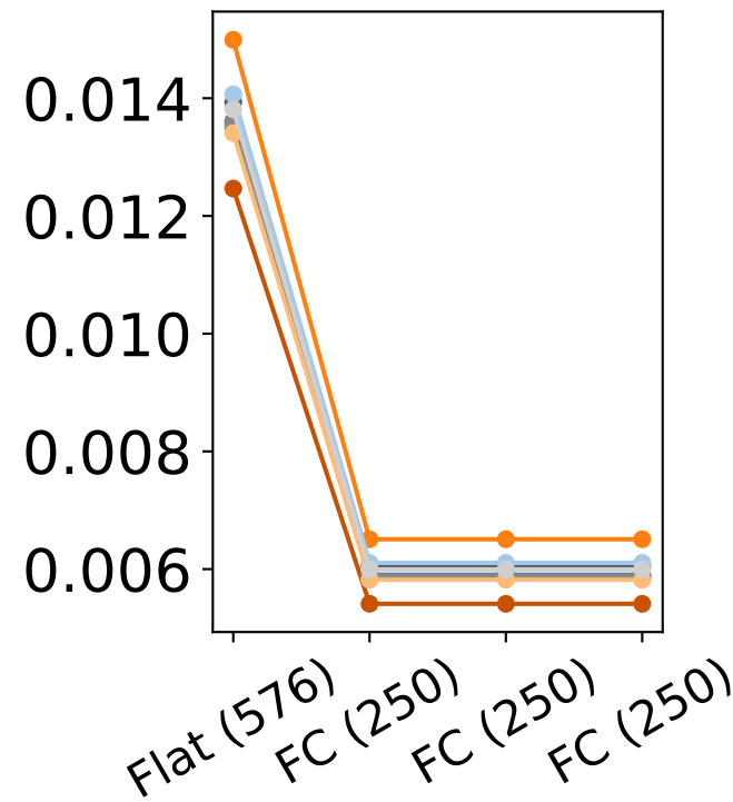
AlexNet-Tiny ImageNet
