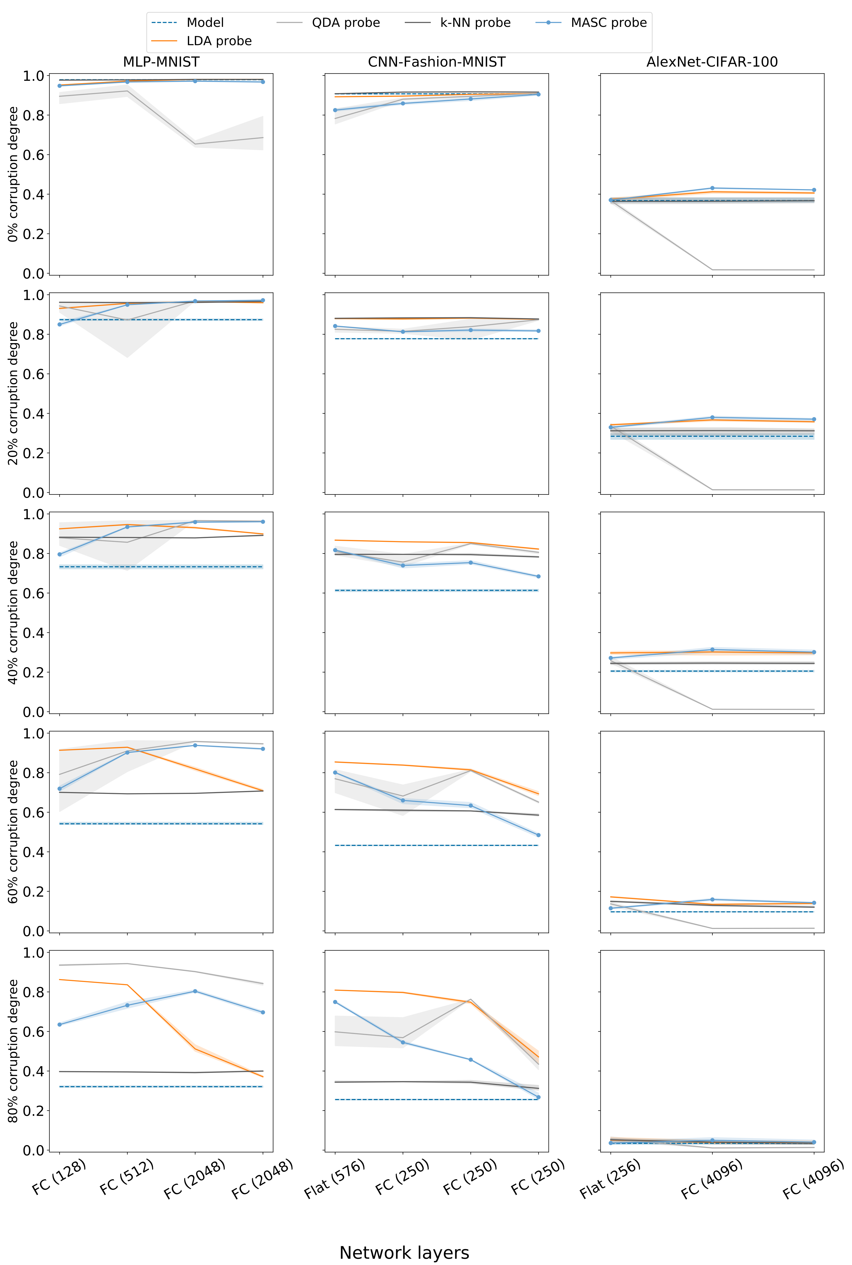
Test Accuracy
