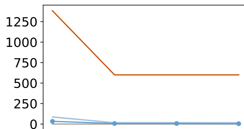
CNN-Fashion-MNIST
