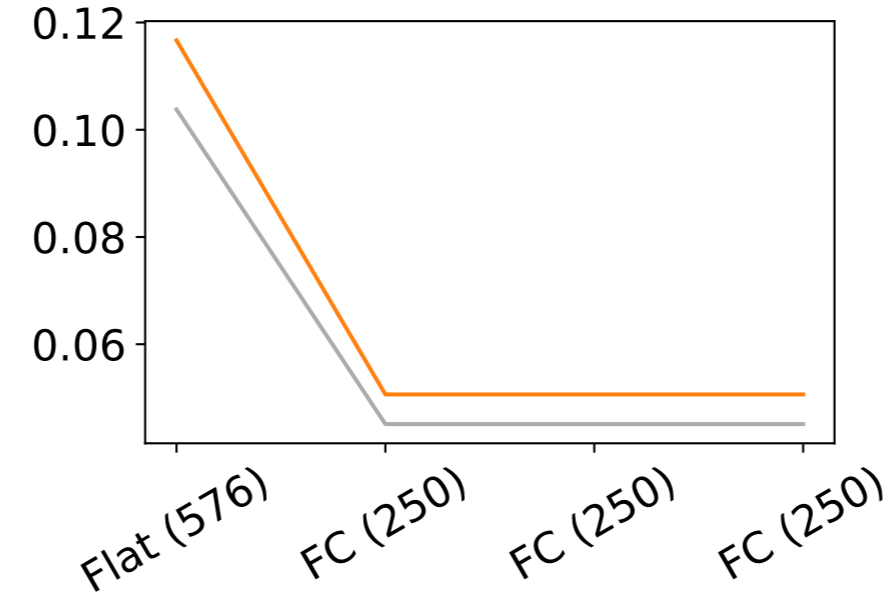
Network layers
