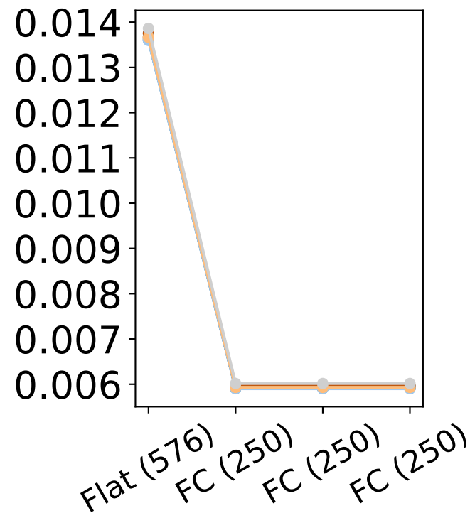
CNN-Fashion-MNIST
