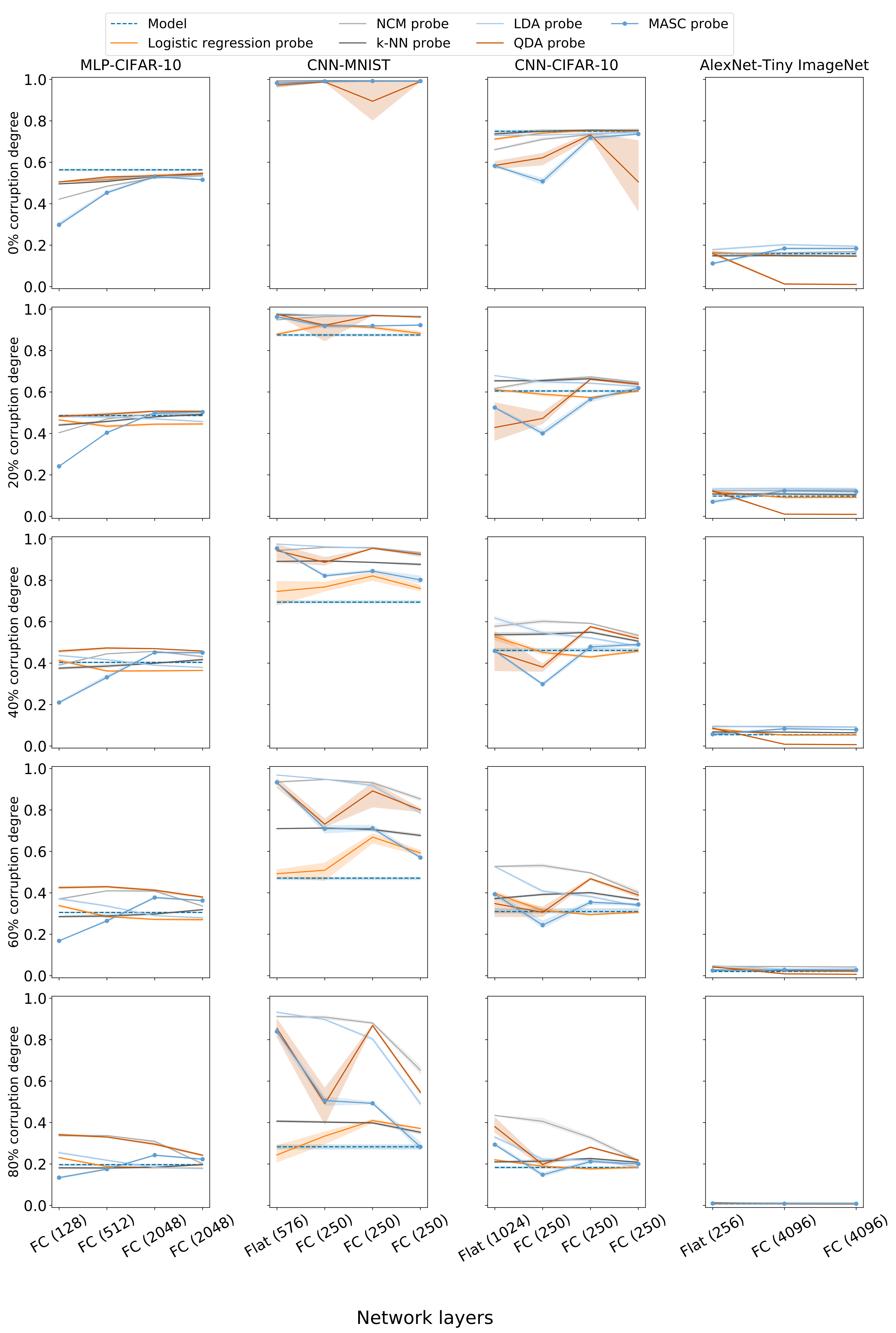
Test Accuracy
