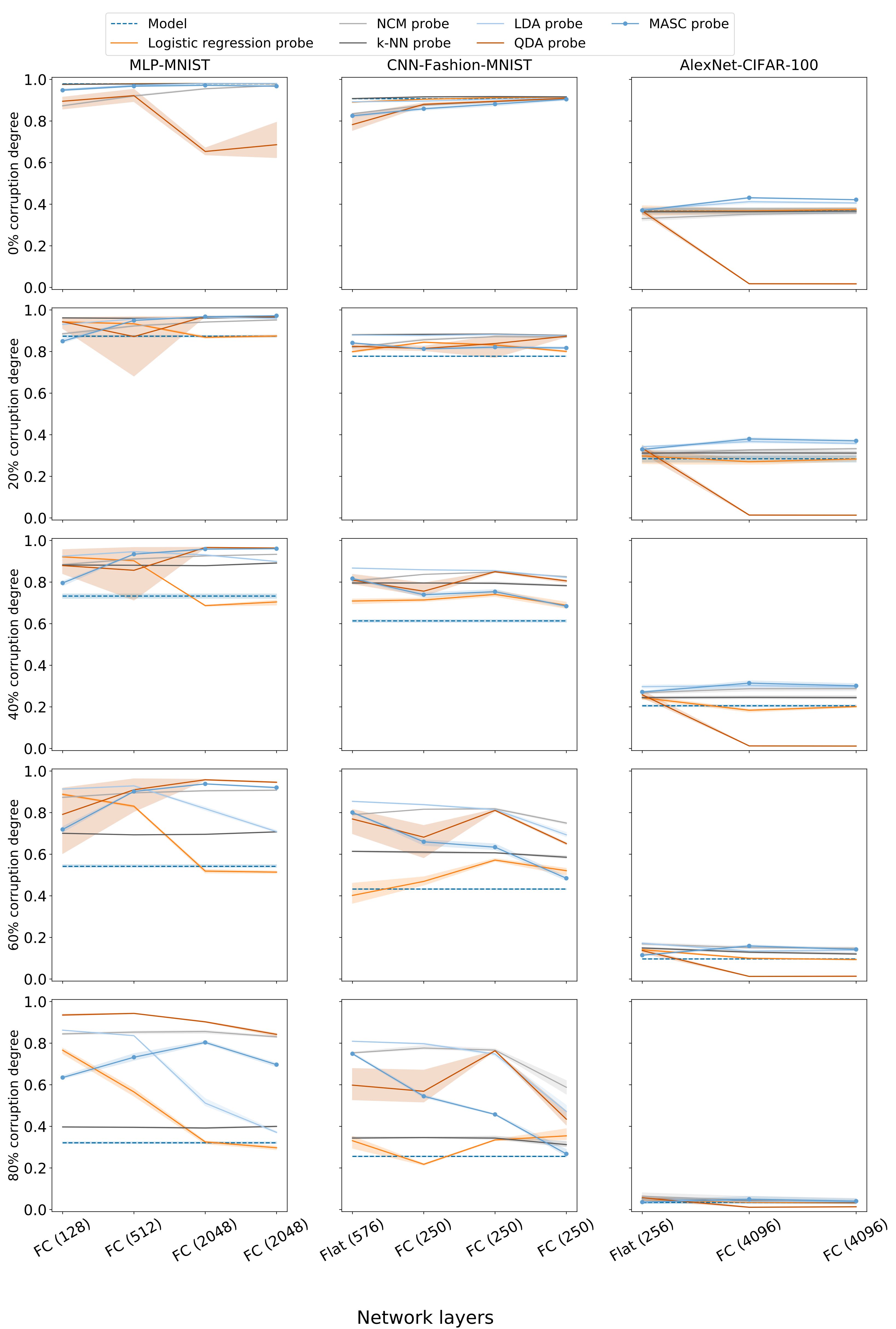
Test Accuracy
