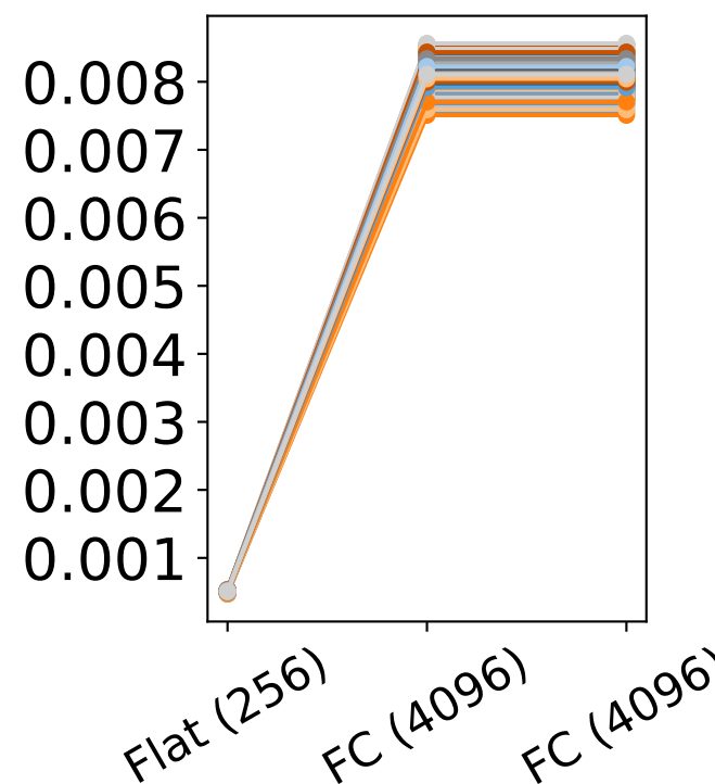
AlexNet-Tiny ImageNet
