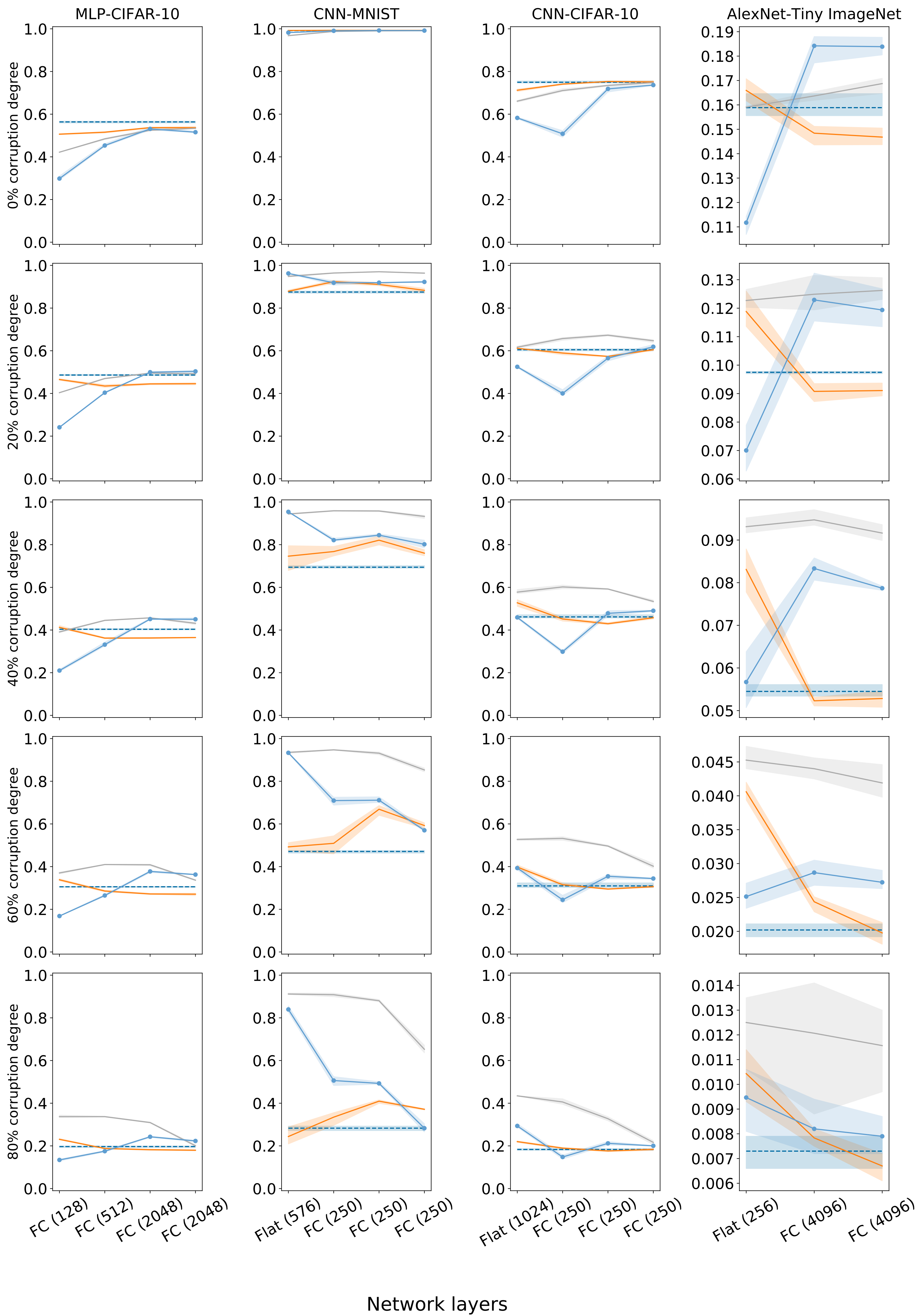
Test Accuracy
