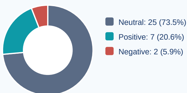
Sentiment Distribution
